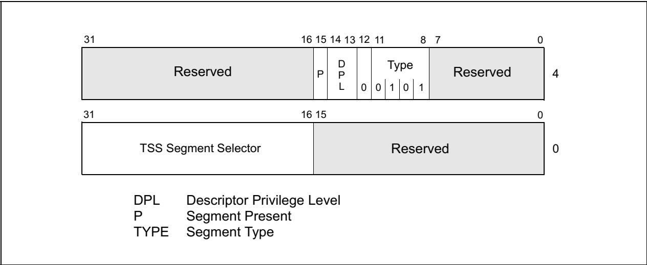
Figure 6-6. Task-Gate Descriptor
