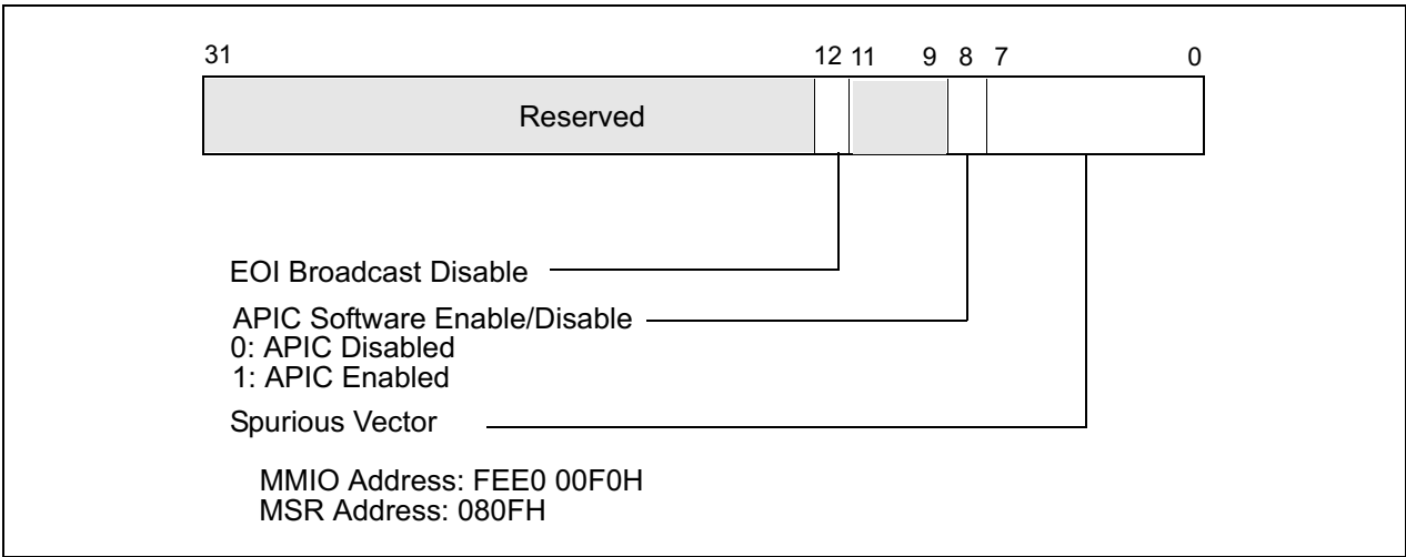
Figure 9-9. Spurious Interrupt Vector Register (SVR) of x2APIC
