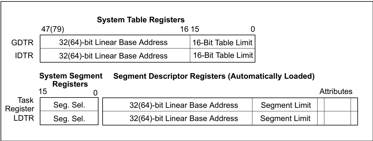
Figure 2-5. Memory Management Registers
