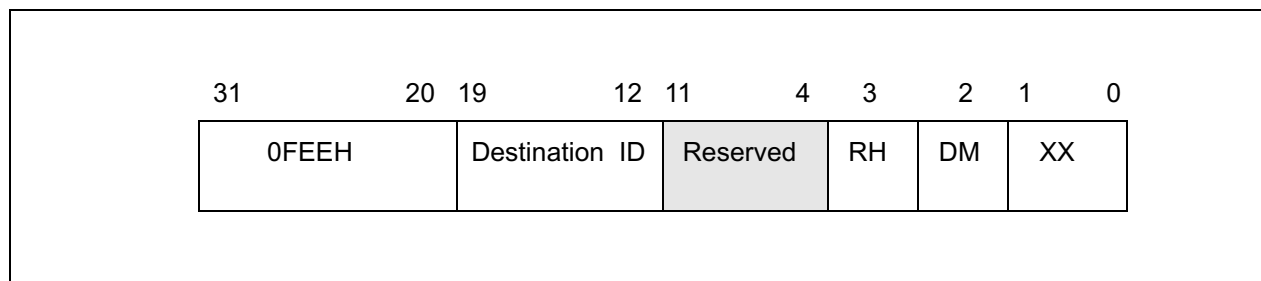
Figure 9-32. Layout of the MSI Message Address Register
