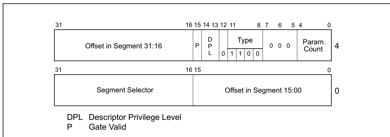
Figure 4-8. Call-Gate Descriptor
