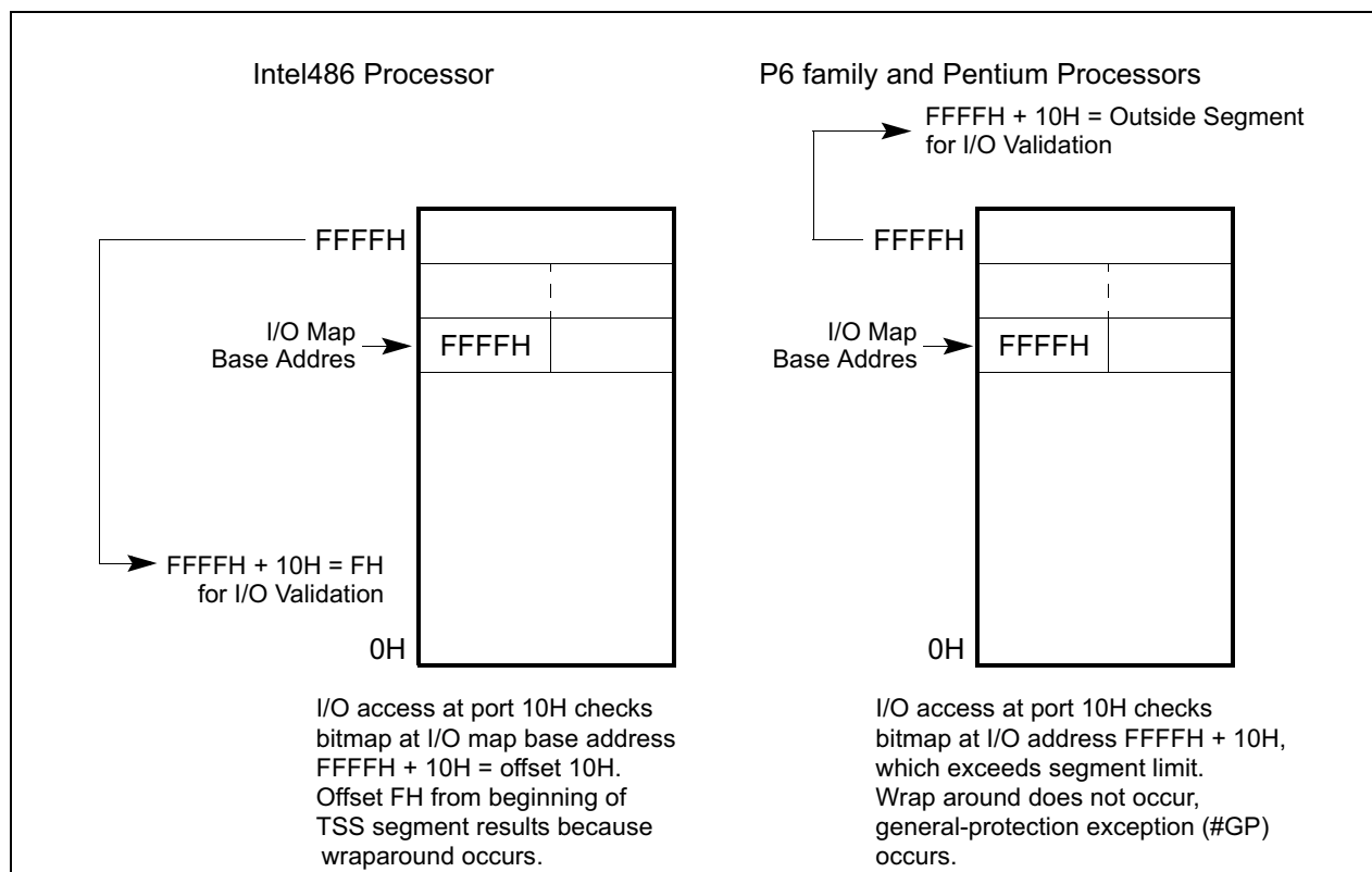
Figure 17-1. I/O Map Base Address Differences
