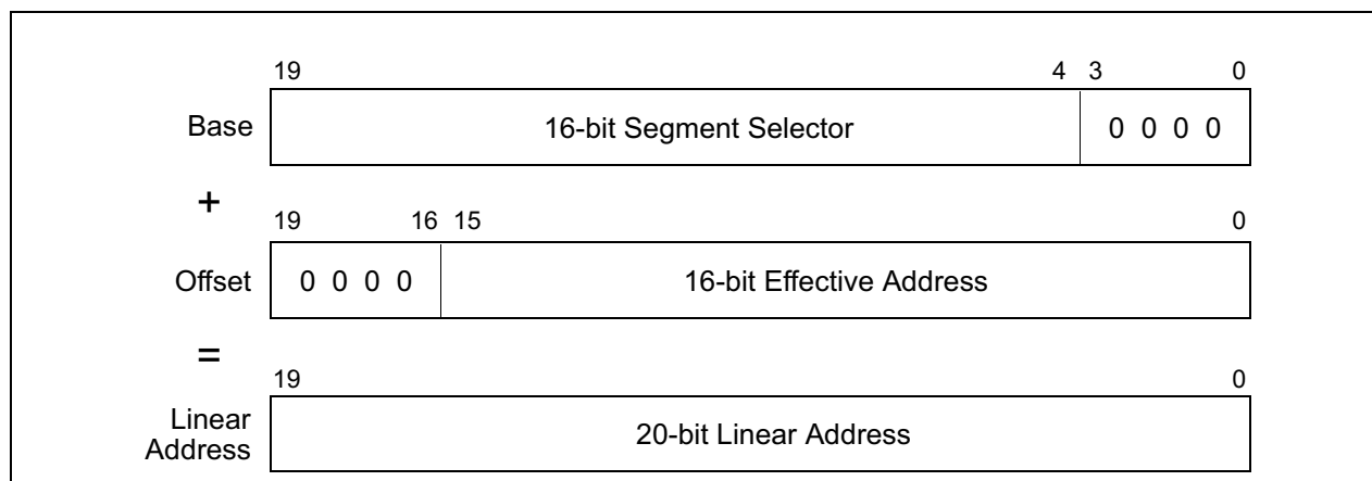
Figure 15-1. Real-Address Mode Address Translation
