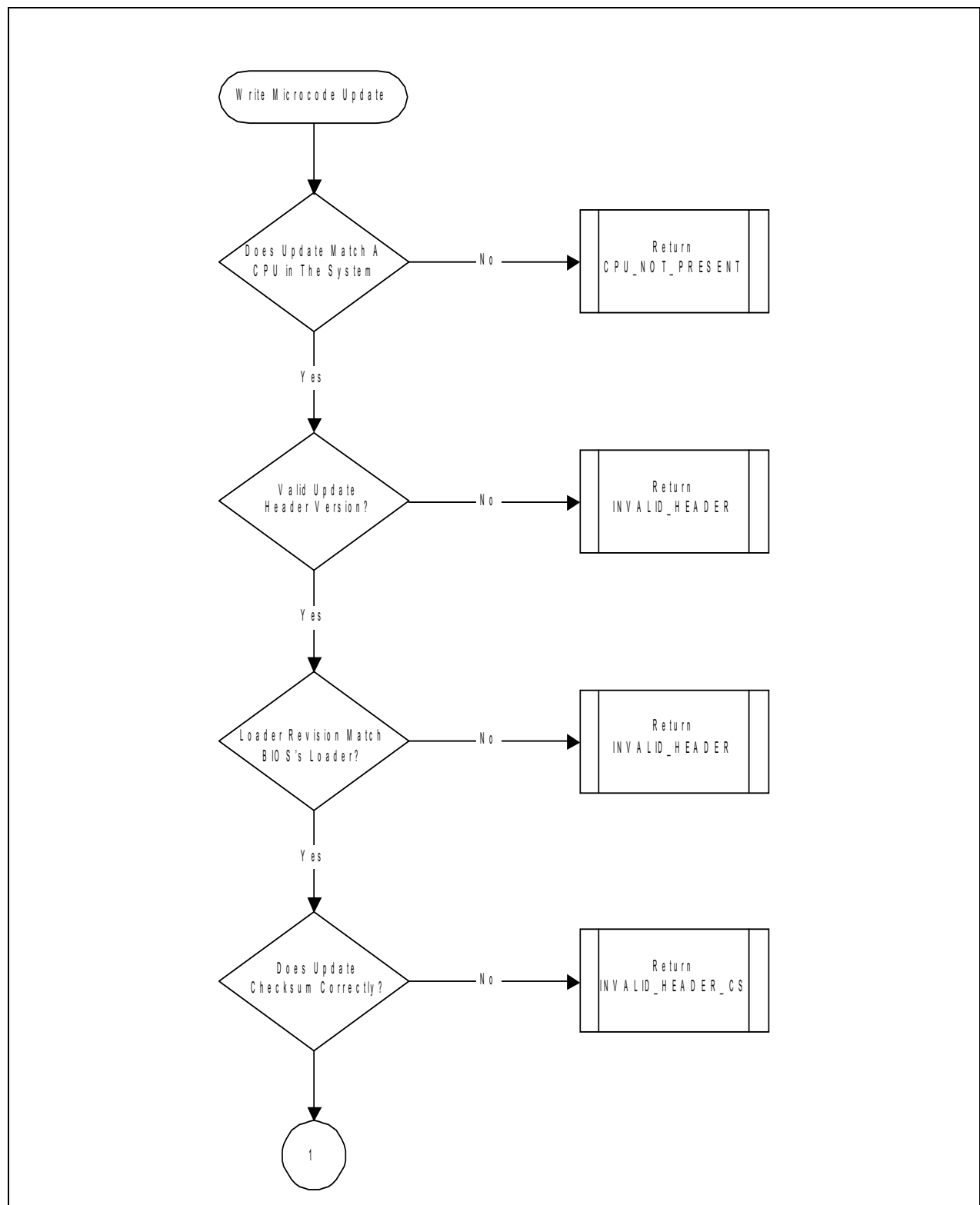
Figure 8-8. Microcode Update Write Operation Flow [1]
