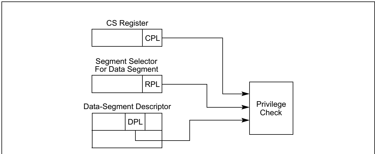
Figure 4-4. Privilege Check for Data Access
