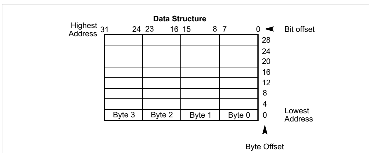
Figure 1-1. Bit and Byte Order
