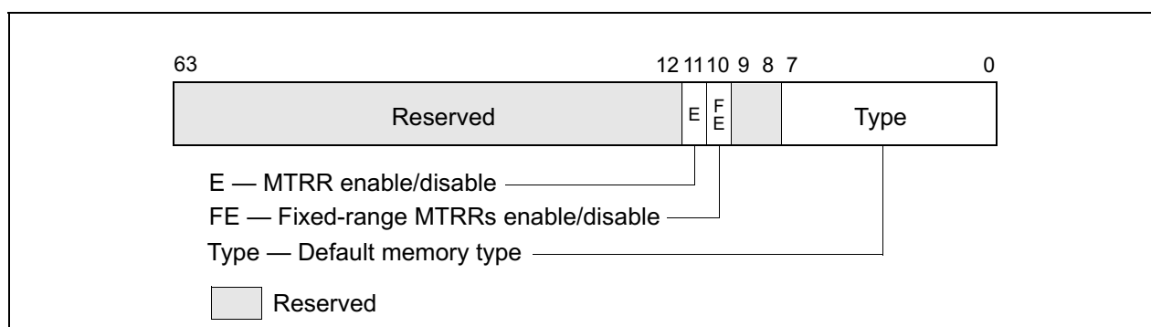
Figure 10-6. IA32_MTRR_DEF_TYPE MSR
