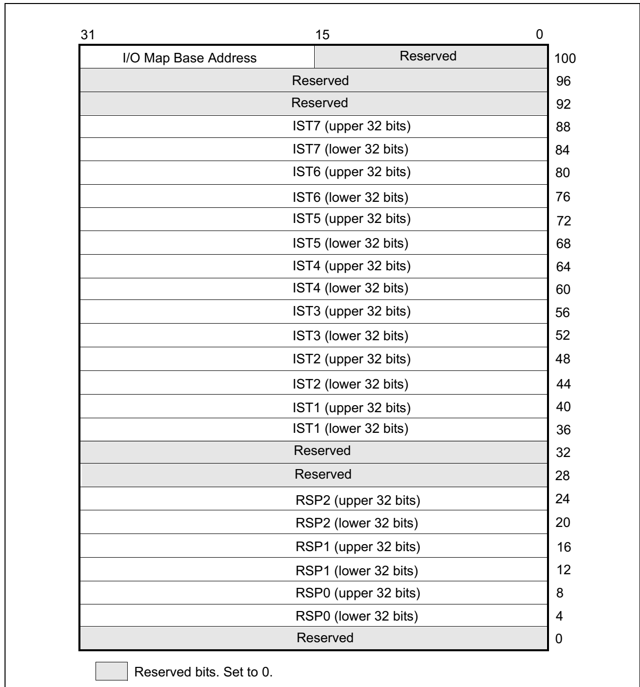
Figure 6-11. 64-Bit TSS Format
