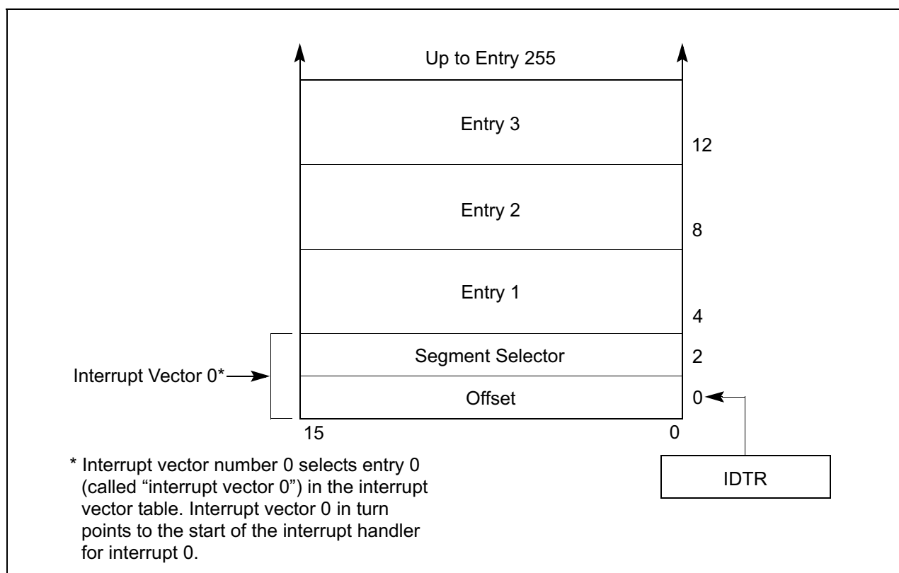
Figure 15-2. Interrupt Vector Table in Real-Address Mode
