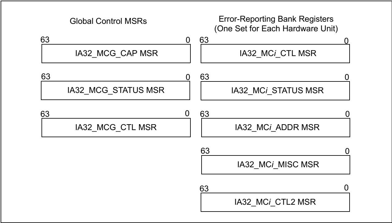
Figure 14-1. Machine-Check MSRs
