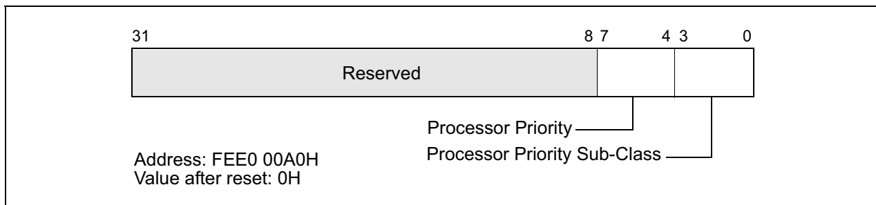
Figure 9-27. Processor Priority Register (PPR)
