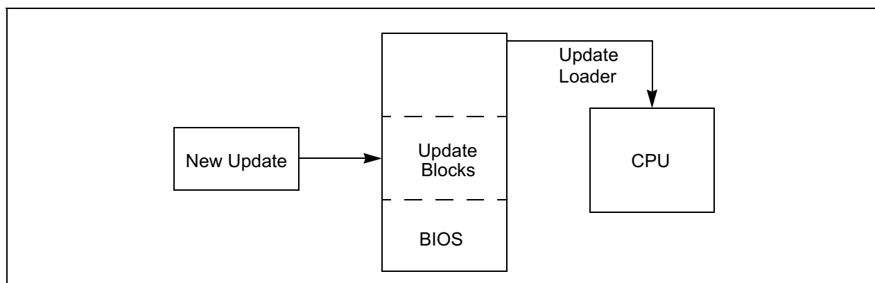
Figure 8-7. Applying Microcode Updates
