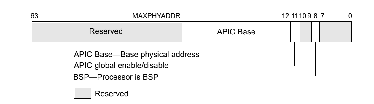
Figure 9-5. IA32_APIC_BASE MSR (APIC_BASE_MSR in P6 Family)
