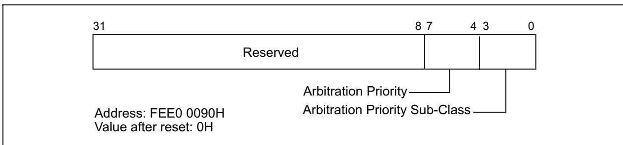
Figure 9-22. Arbitration Priority Register (APR)
