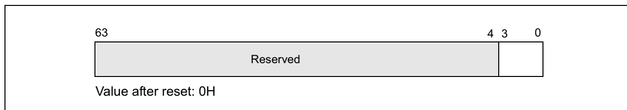
Figure 9-30. CR8 Register
