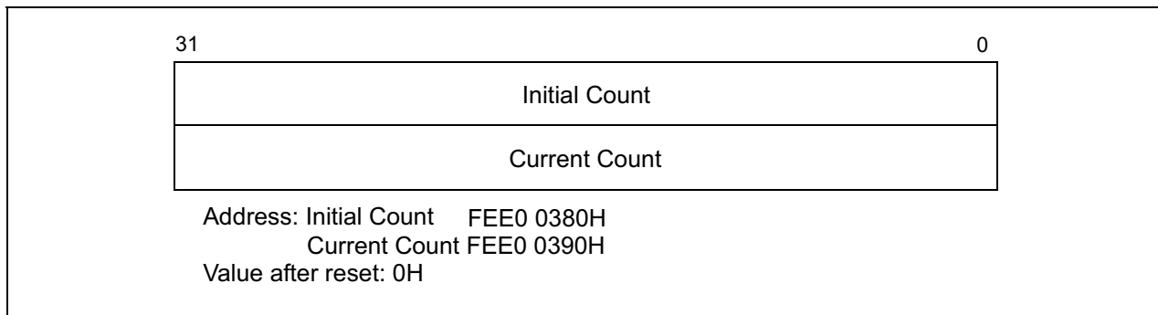
Figure 9-16. Initial Count and Current Count Registers
