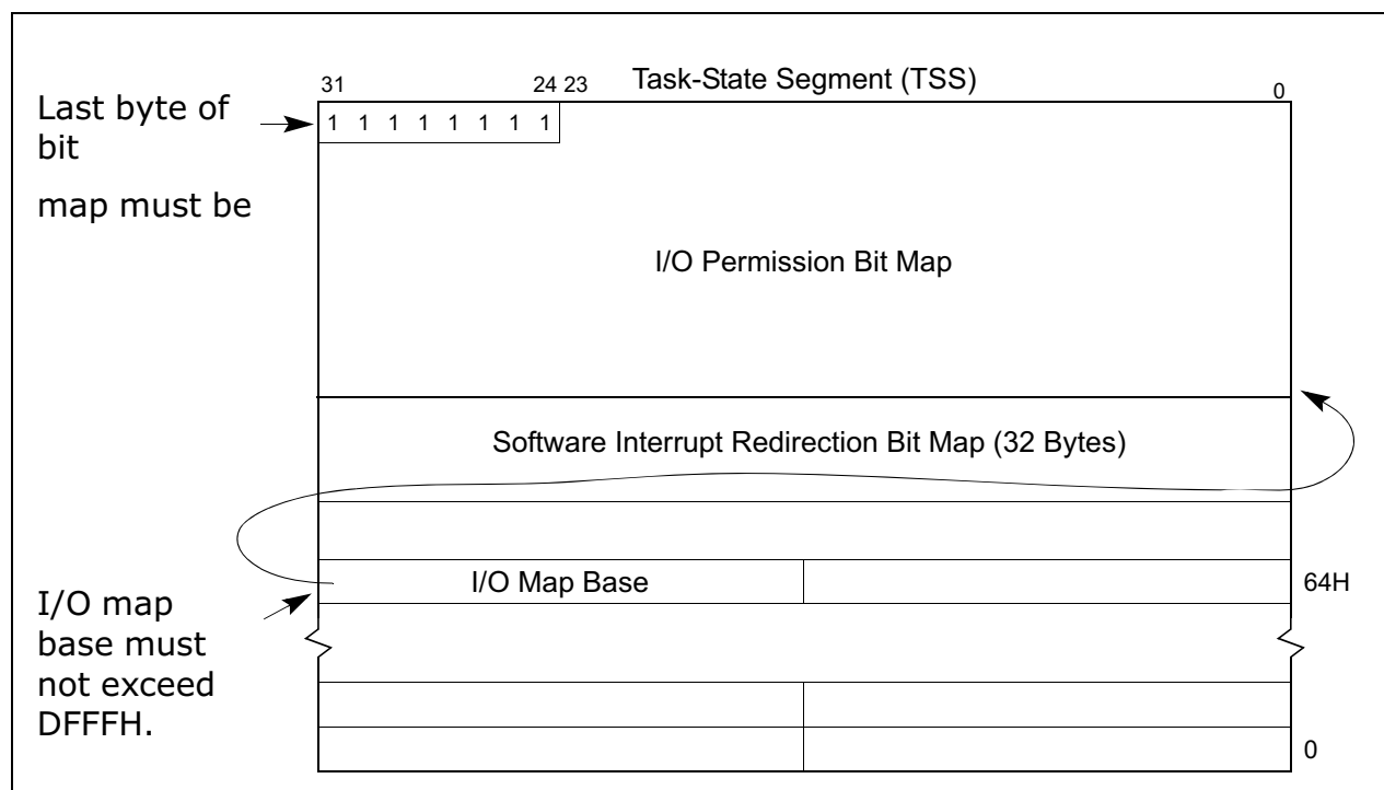
Figure 15-5. Software Interrupt Redirection Bit Map in TSS
