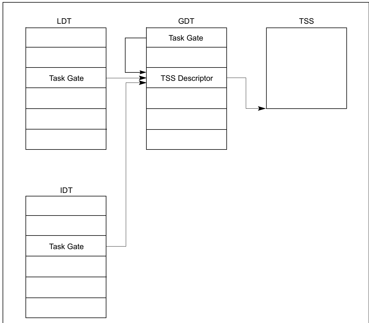
Figure 6-7. Task Gates Referencing the Same Task
