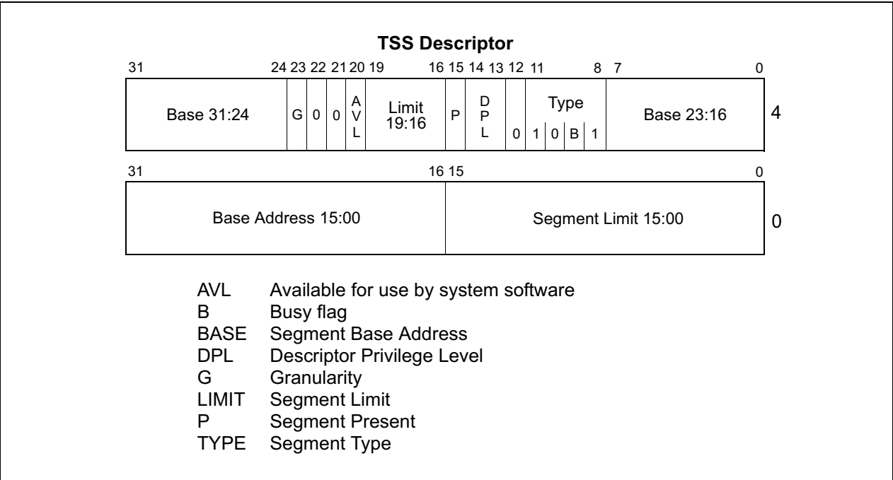
Figure 6-3. TSS Descriptor
