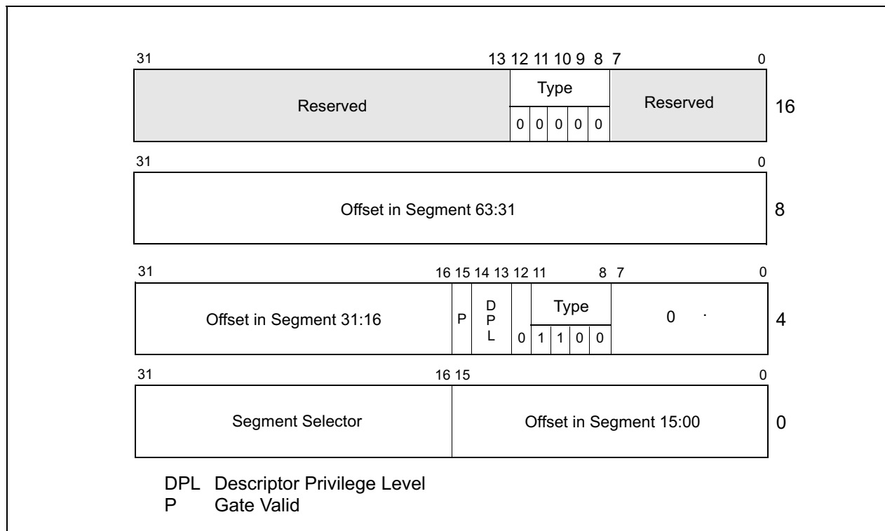
Figure 4-9. Call-Gate Descriptor in IA-32e Mode
