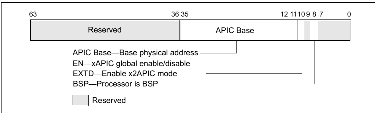
Figure 9-8. IA32_APIC_BASE MSR Supporting x2APIC
