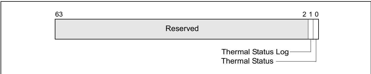
Figure 13-7. IA32_THERM_STATUS MSR
