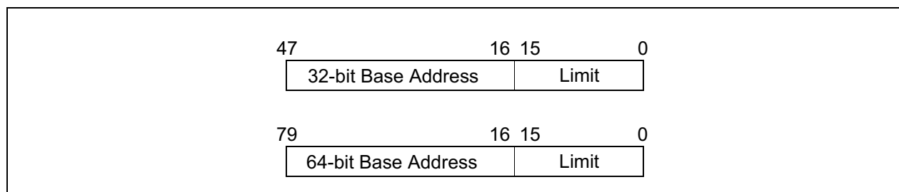
Figure 3-11. Pseudo-Descriptor Formats
