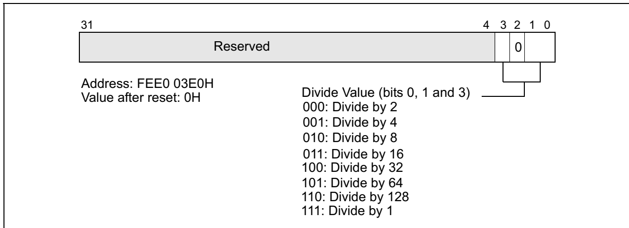
Figure 9-15. Divide Configuration Register
