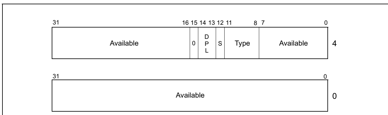
Figure 3-9. Segment Descriptor When Segment-Present Flag Is Clear
