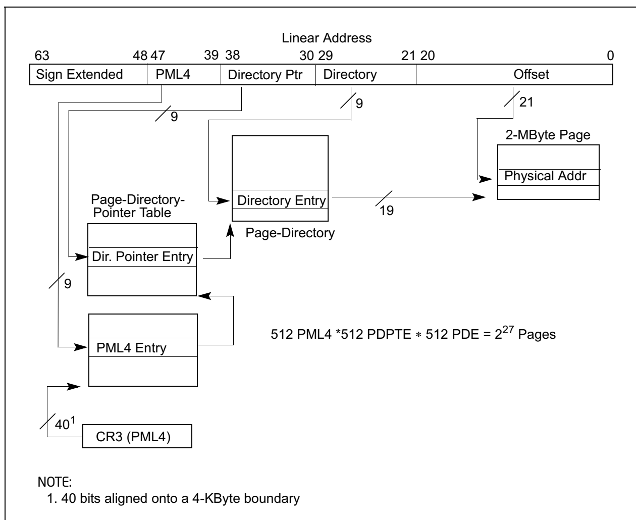
Figure 3-25. IA-32e Mode Paging Structures (2-MByte pages)
