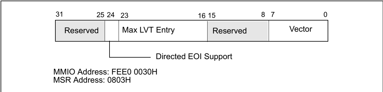
Figure 9-10. Local APIC Version Register of x2APIC
