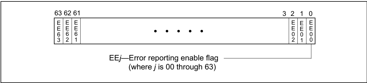
Figure 14-4. IA32_MCi_CTL Register
