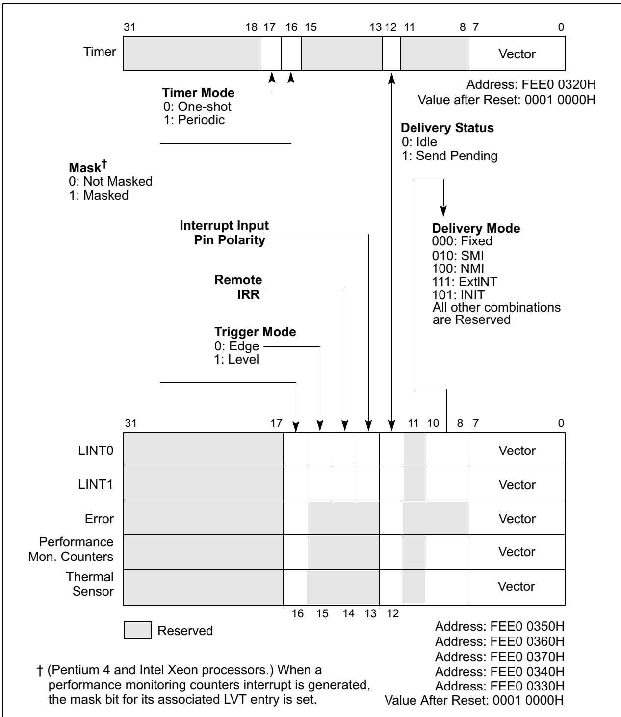
Figure 9-12. Local Vector Table (LVT)
