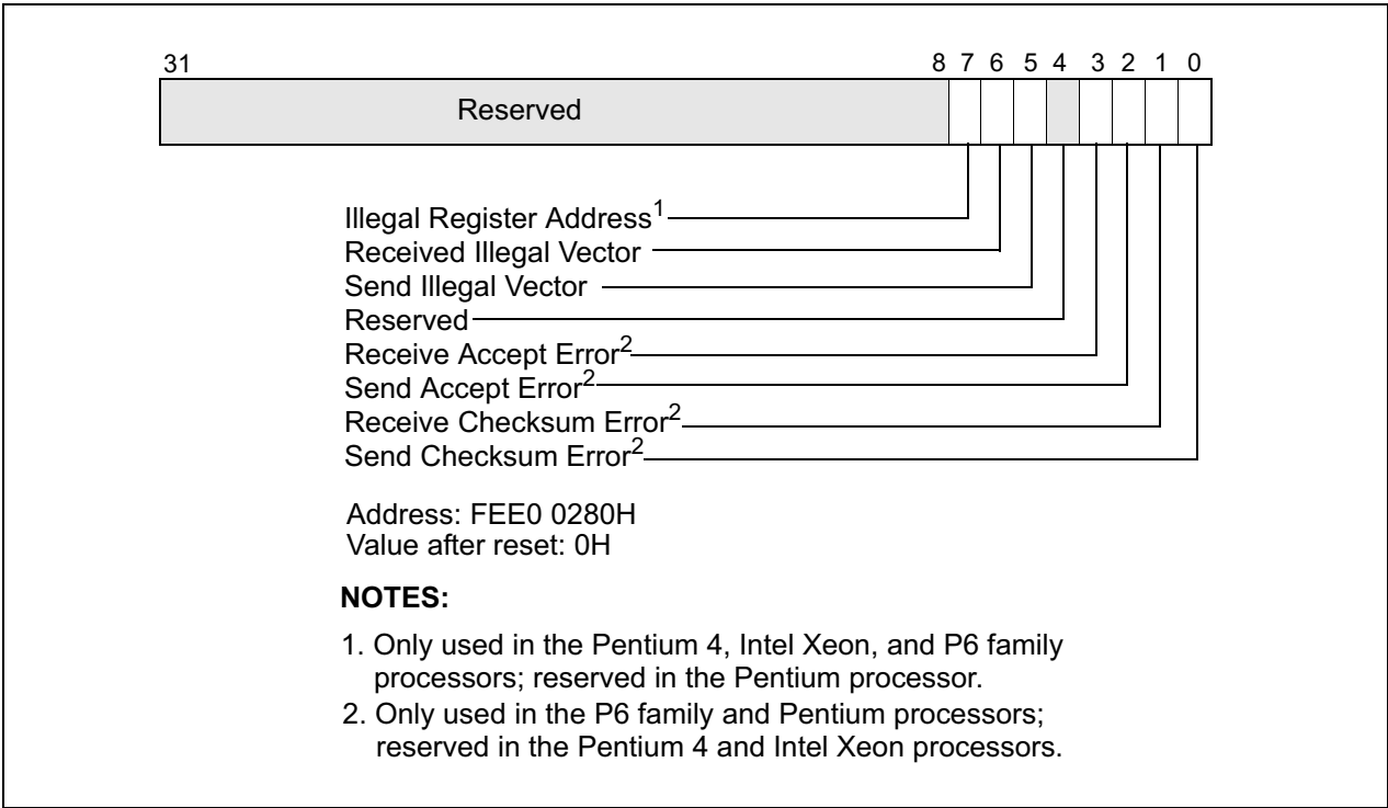
Figure 9-13. Error Status Register (ESR)
