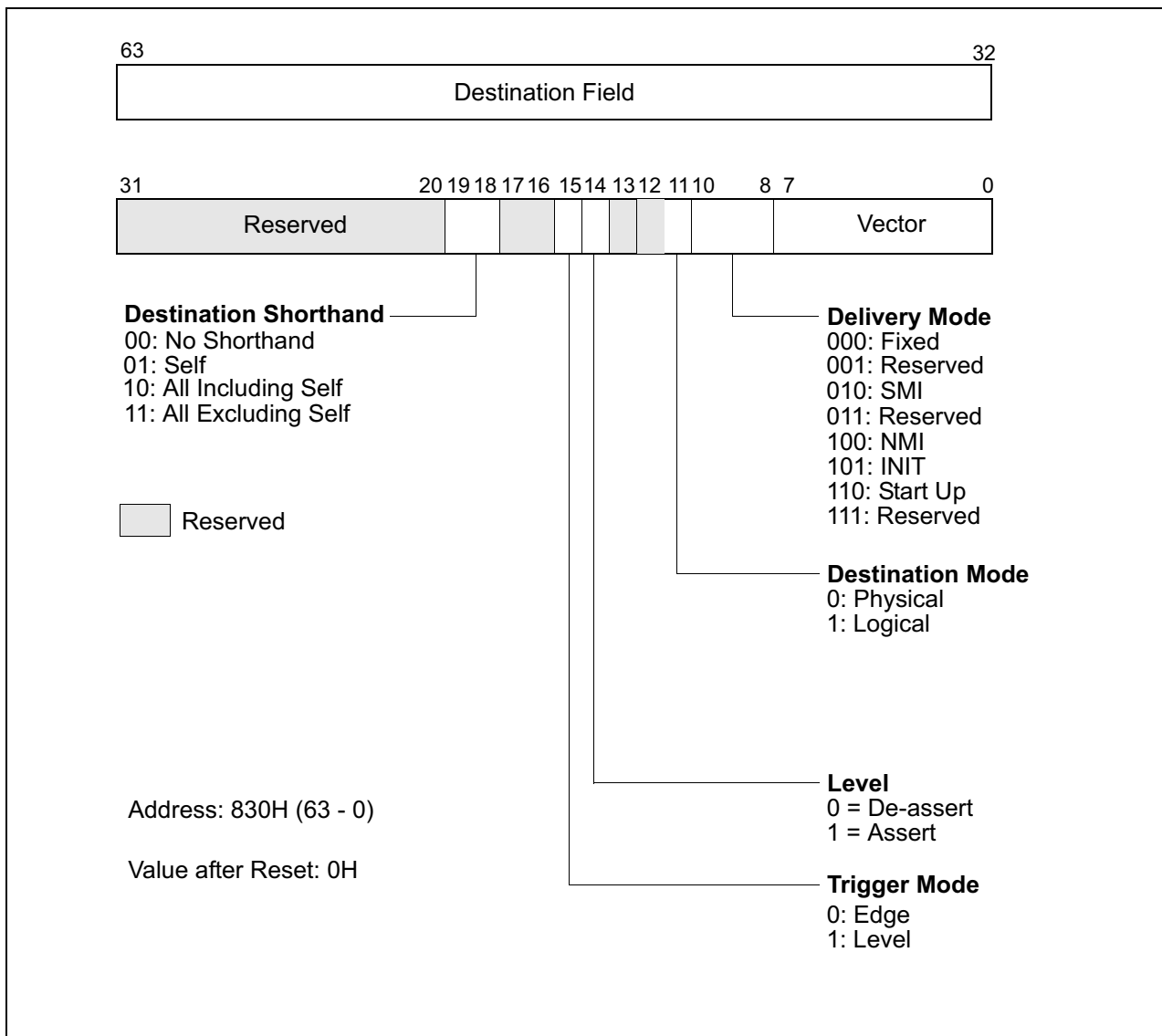
Figure 9-18. Interrupt Command Register (ICR) in x2APIC Mode
