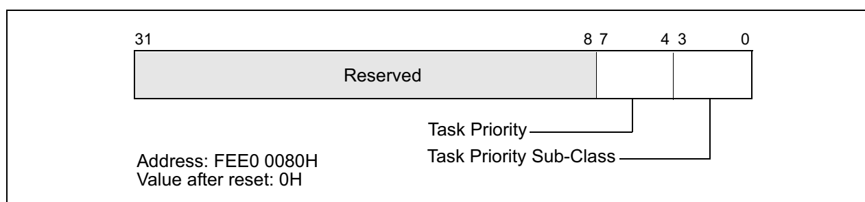
Figure 9-26. Task Priority Register (TPR)
