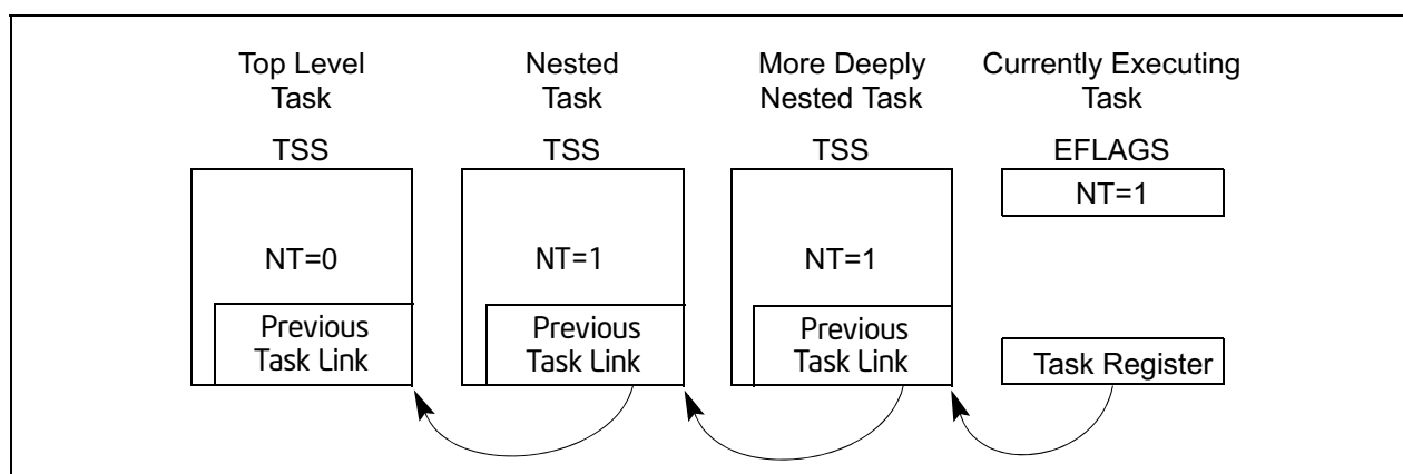
Figure 6-8. Nested Tasks
