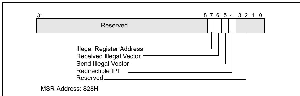
Figure 9-14. Error Status Register (ESR) in x2APIC Mode
