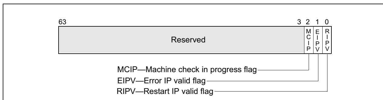
Figure 14-3. IA32_MCG_STATUS Register
