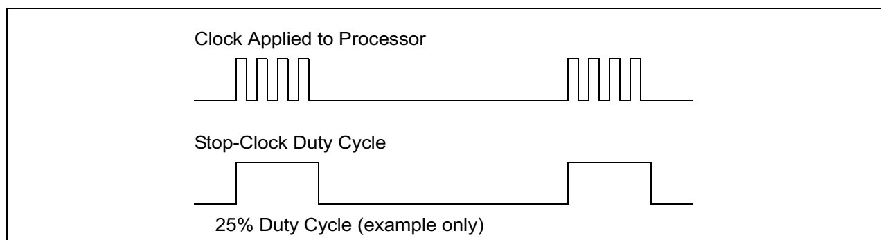
Figure 13-4. Processor Modulation Through Stop-Clock Mechanism
