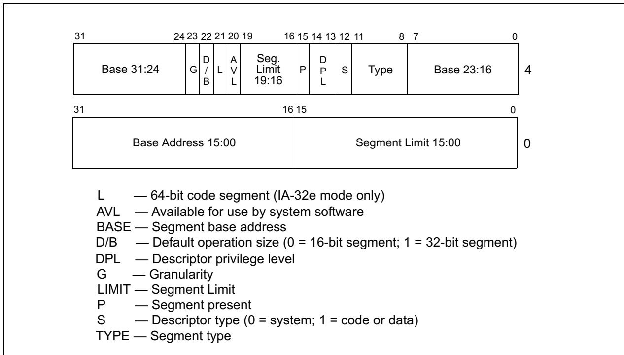
Figure 3-8. Segment Descriptor
