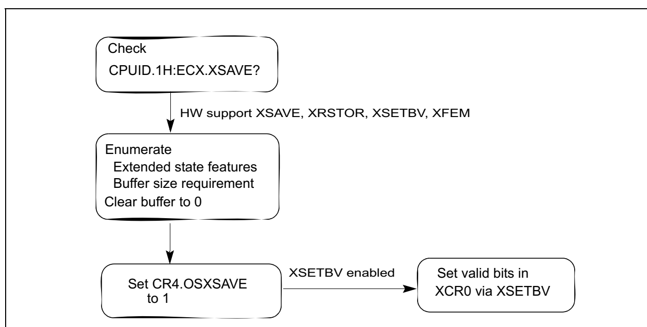
Figure 12-3. OS Enabling of Processor Extended State Support
