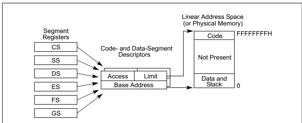
Figure 3-2. Flat Model
