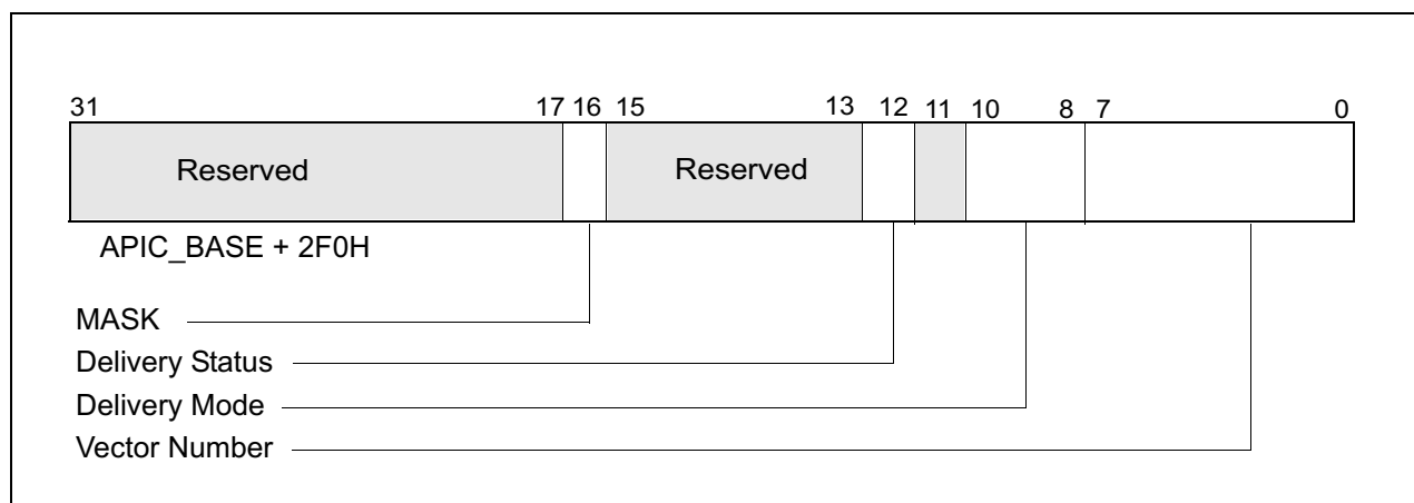
Figure 14-9. Local APIC CMCI LVT Register
