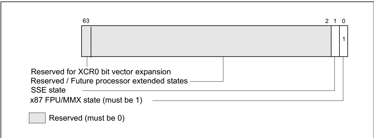
Figure 2-7. XFEATURE_ENABLED_MASK Register (XCR0)
