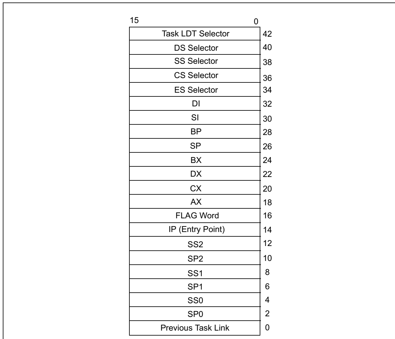
Figure 6-10. 16-Bit TSS Format
