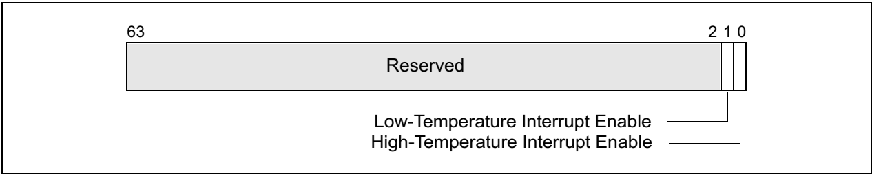
Figure 13-8. IA32_THERM_INTERRUPT MSR
