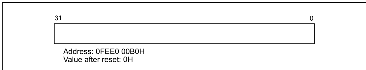
Figure 9-29. EOI Register
