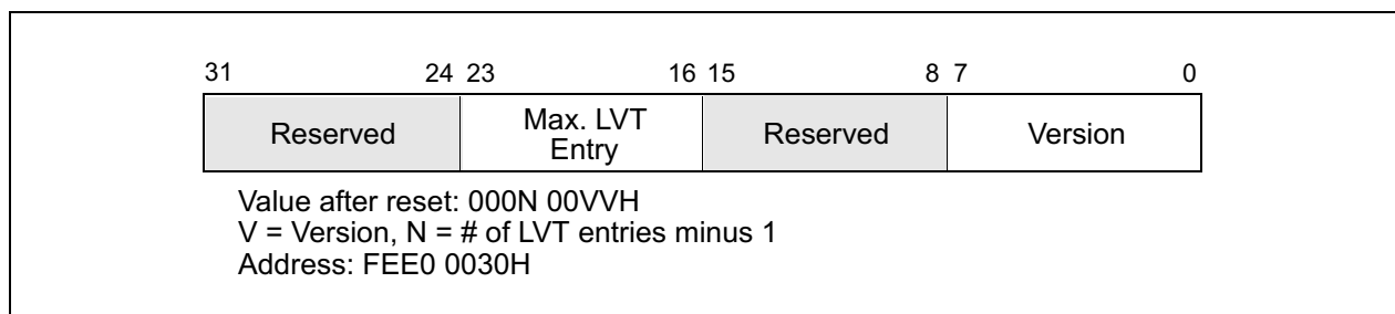
Figure 9-7. Local APIC Version Register
