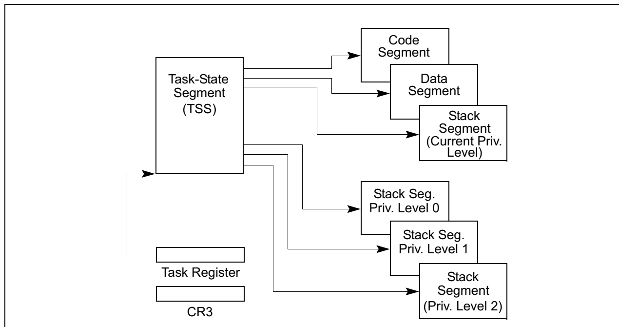
Figure 6-1. Structure of a Task
