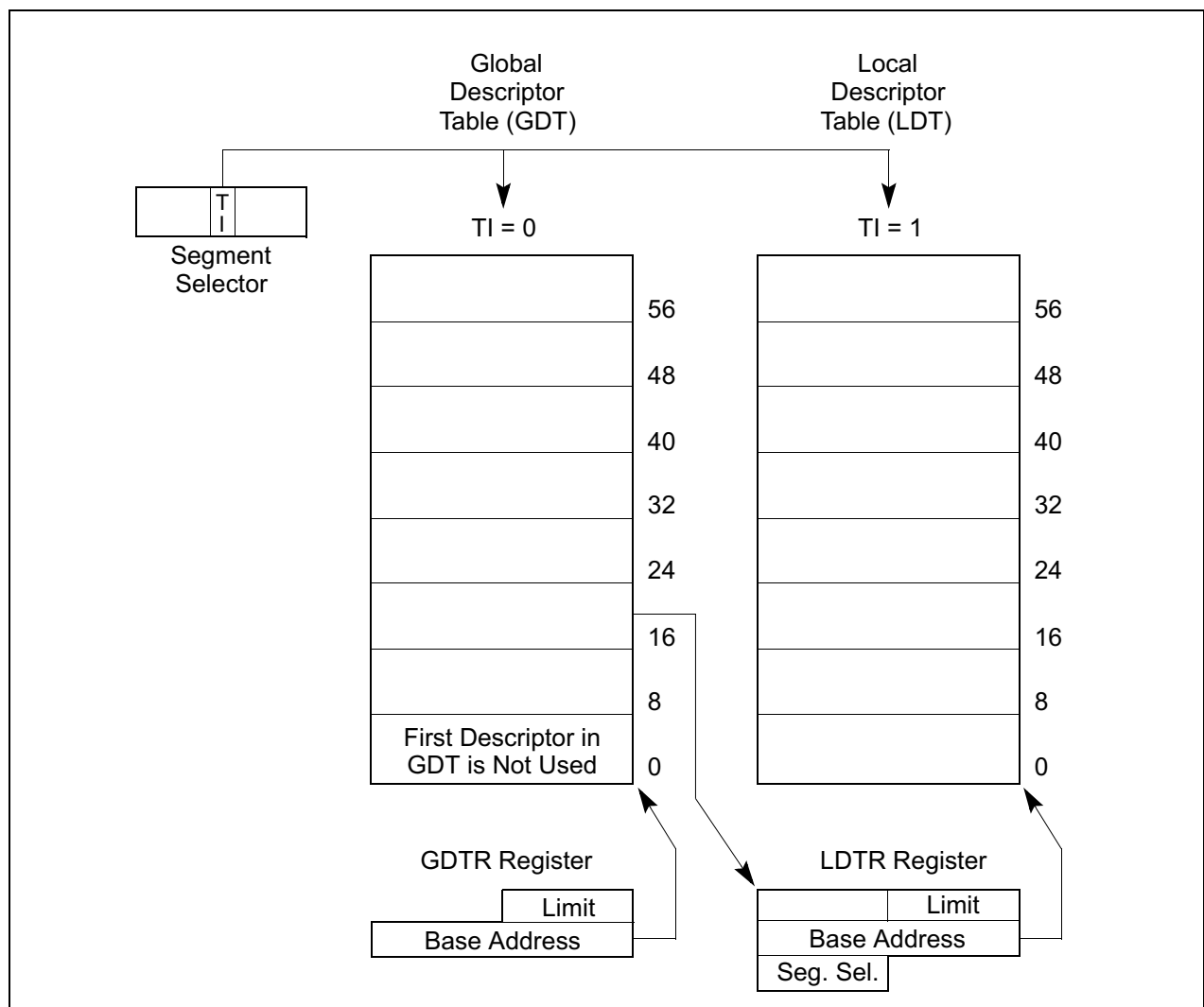
Figure 3-10. Global and Local Descriptor Tables
