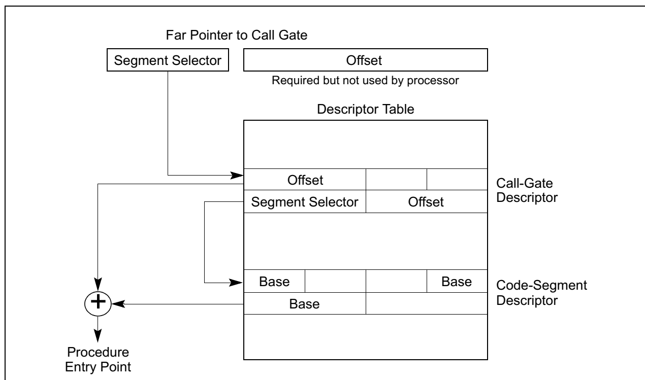
Figure 4-10. Call-Gate Mechanism
