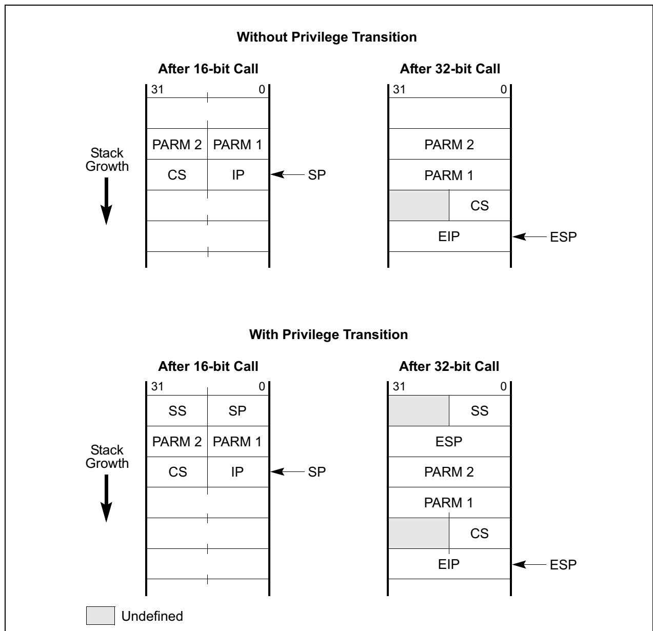
Figure 16-1. Stack after Far 16- and 32-Bit Calls
