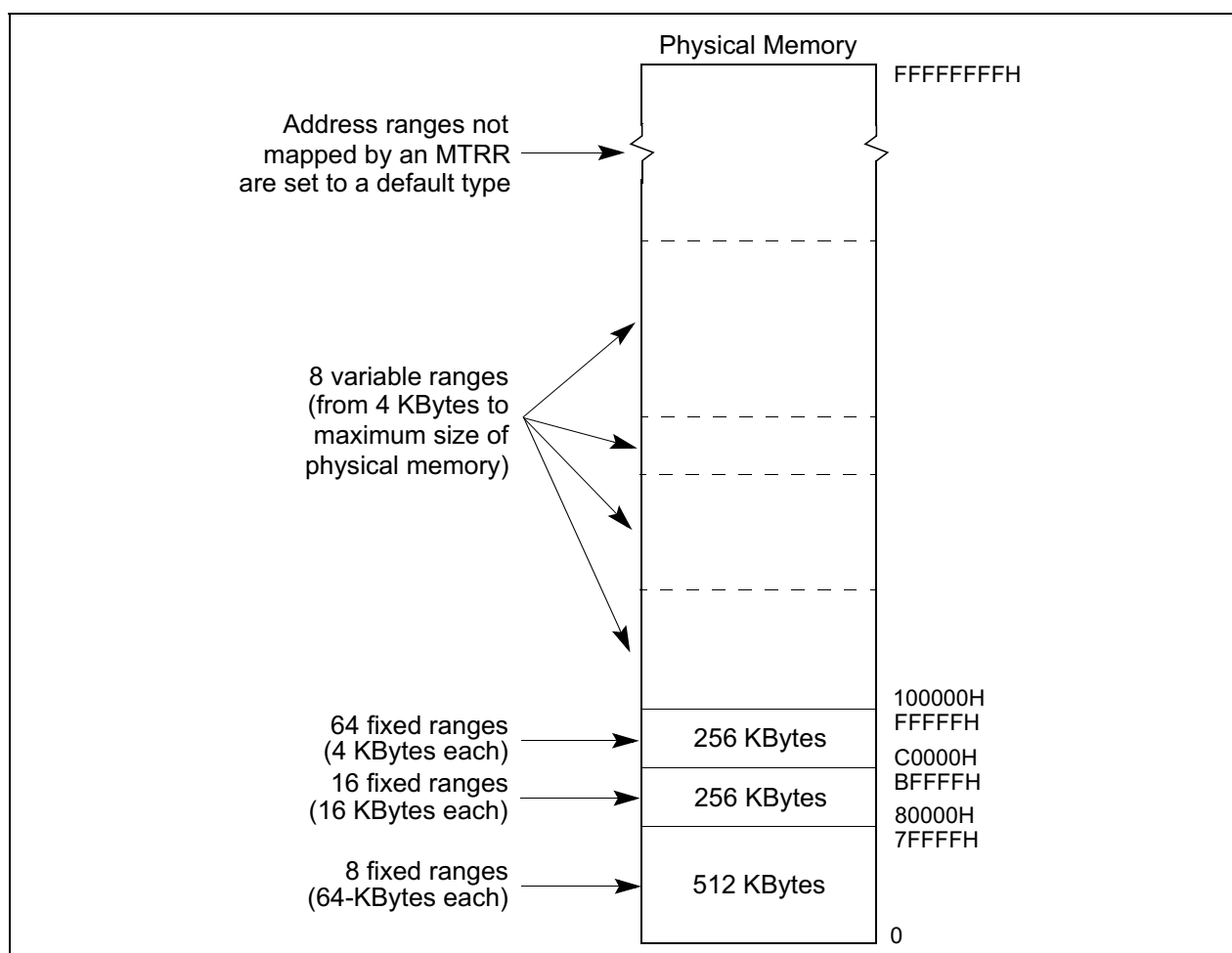
Figure 10-4. Mapping Physical Memory With MTRRs
