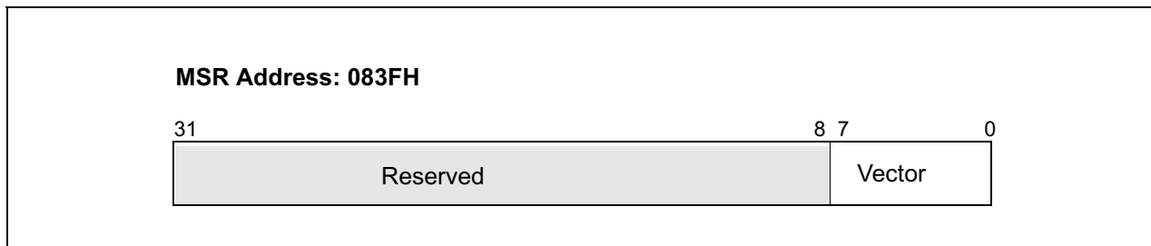
Figure 9-23. SELF IPI register
