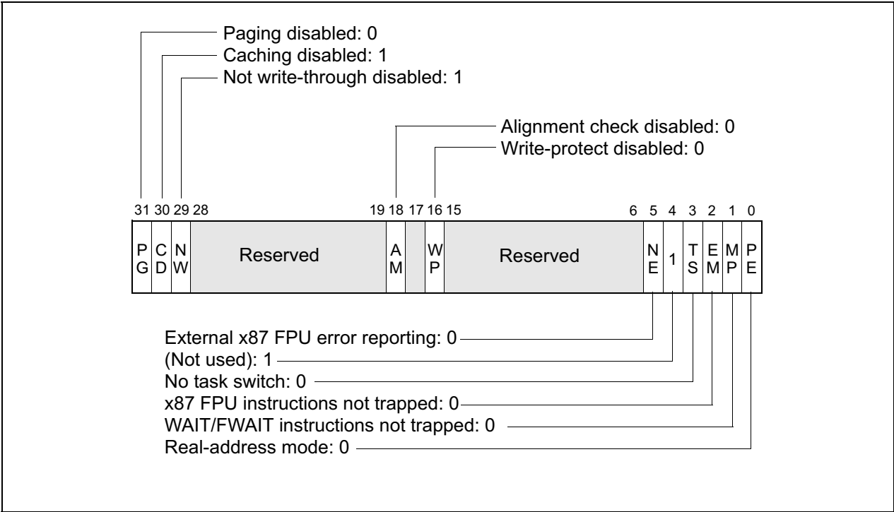
Figure 8-1. Contents of CR0 Register after Reset
