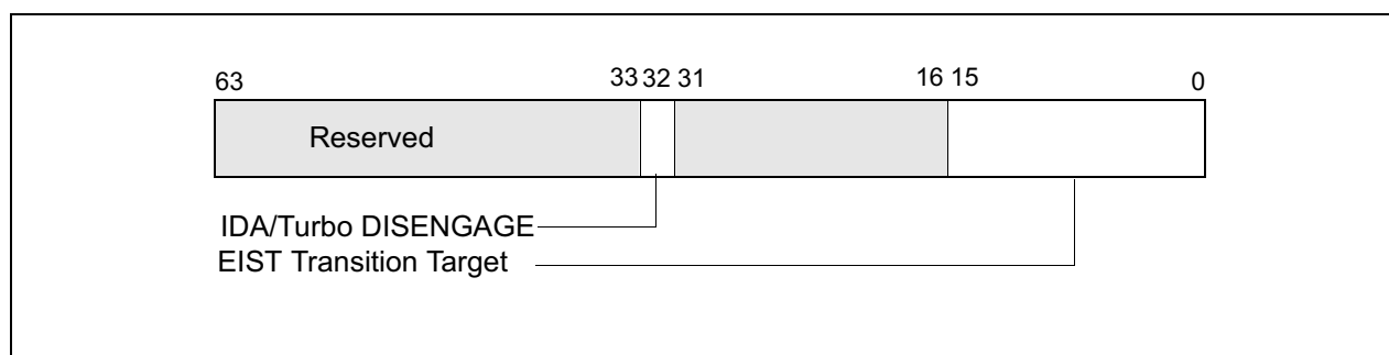
Figure 13-2. IA32_PERF_CTL Register
