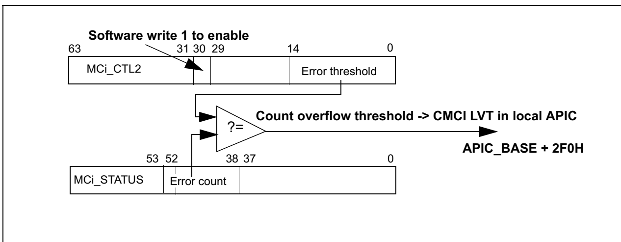
Figure 14-8. CMCI Behavior
