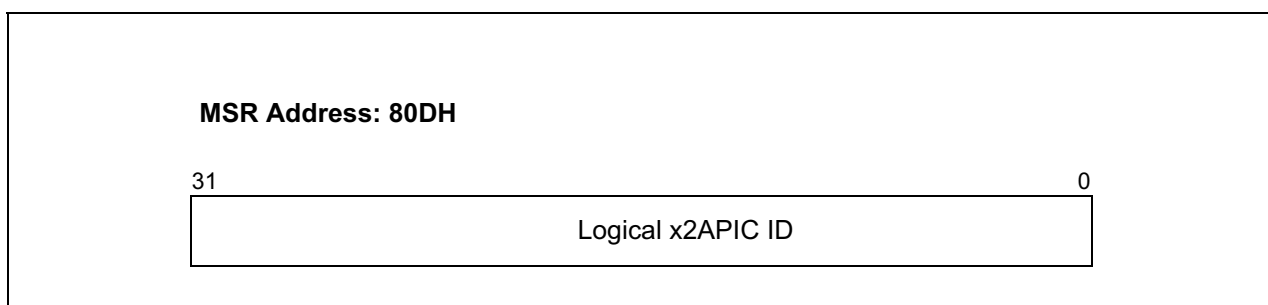
Figure 9-21. Logical Destination Register in x2APIC Mode
