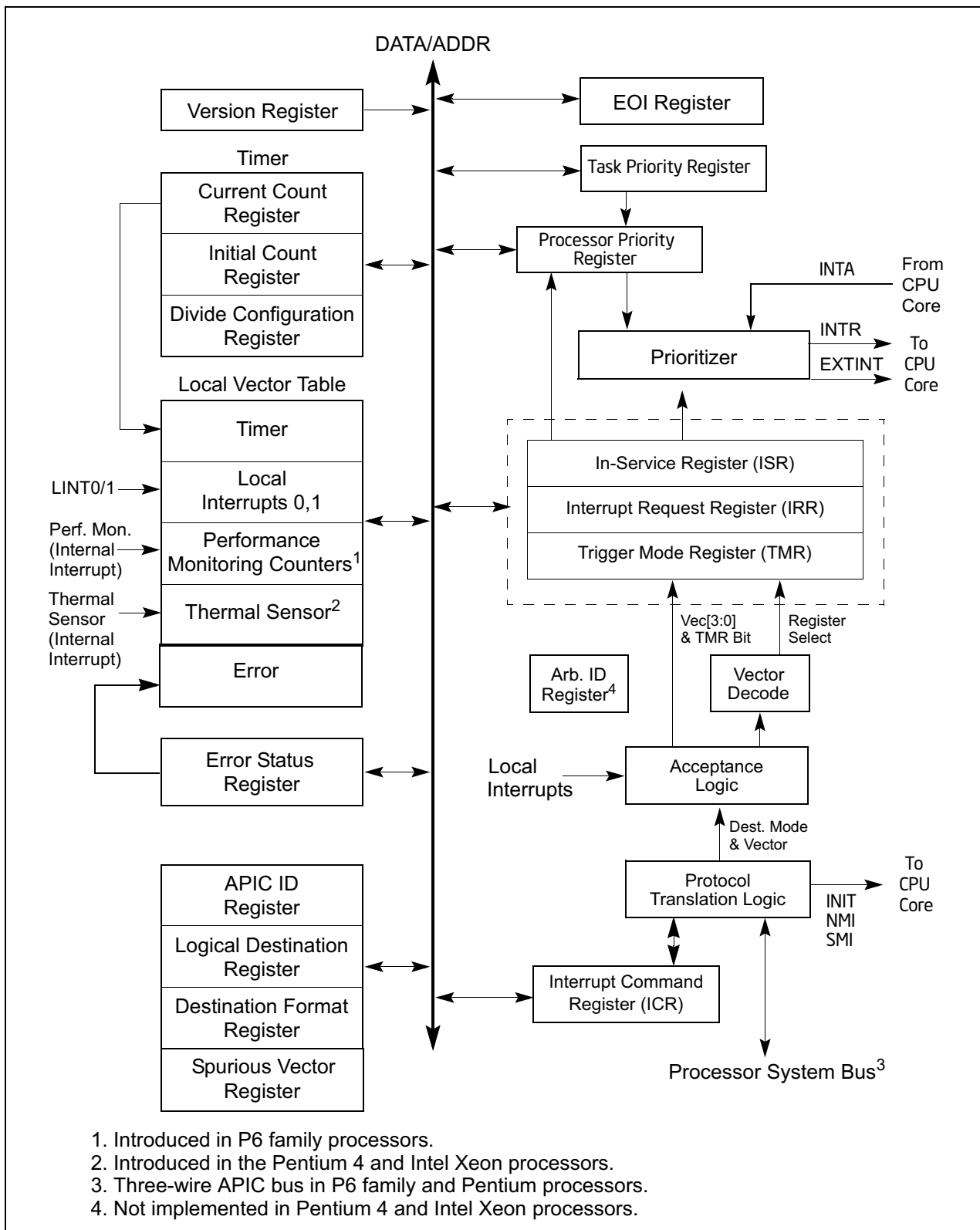
Figure 9-4. Local APIC Structure
