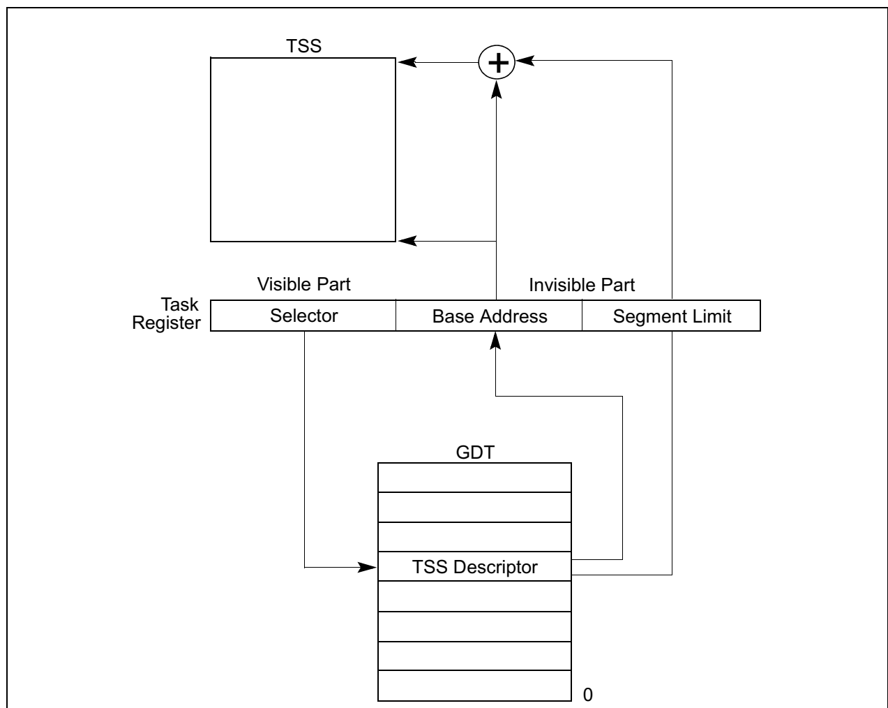
Figure 6-5. Task Register
