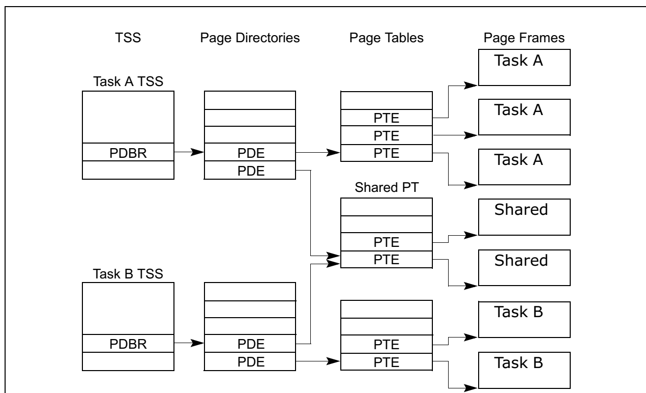
Figure 6-9. Overlapping Linear-to-Physical Mappings
