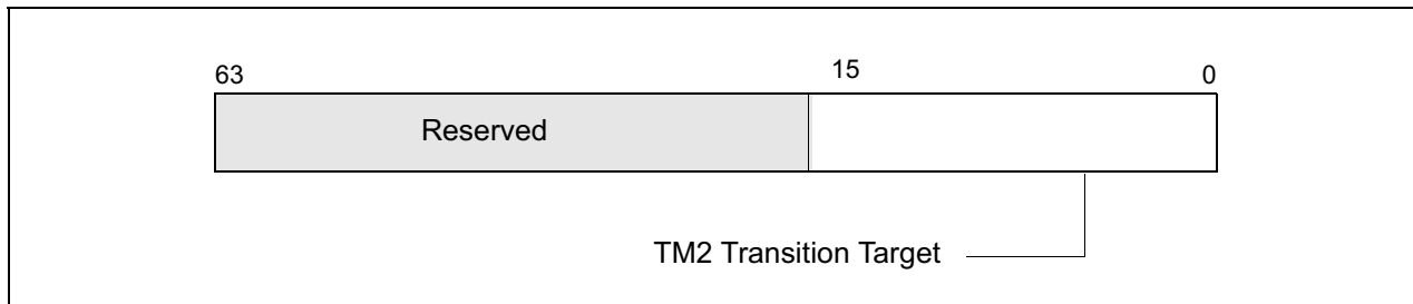
Figure 13-6. MSR_THERM2_CTL Register for Supporting TM2
