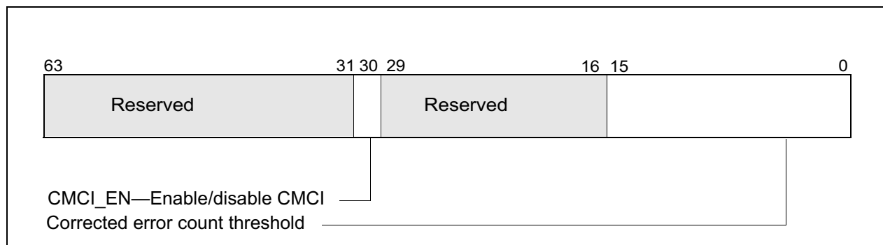
Figure 14-7. IA32_MCi_CTL2 Register
