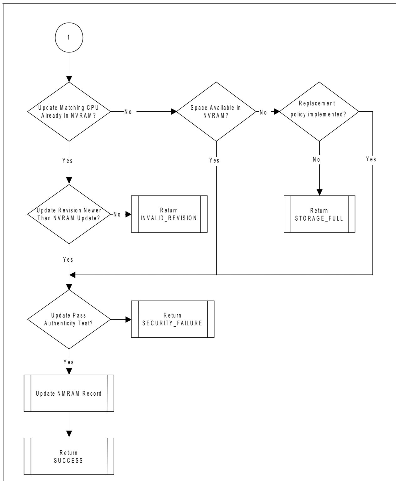
Figure 8-9. Microcode Update Write Operation Flow [2]
