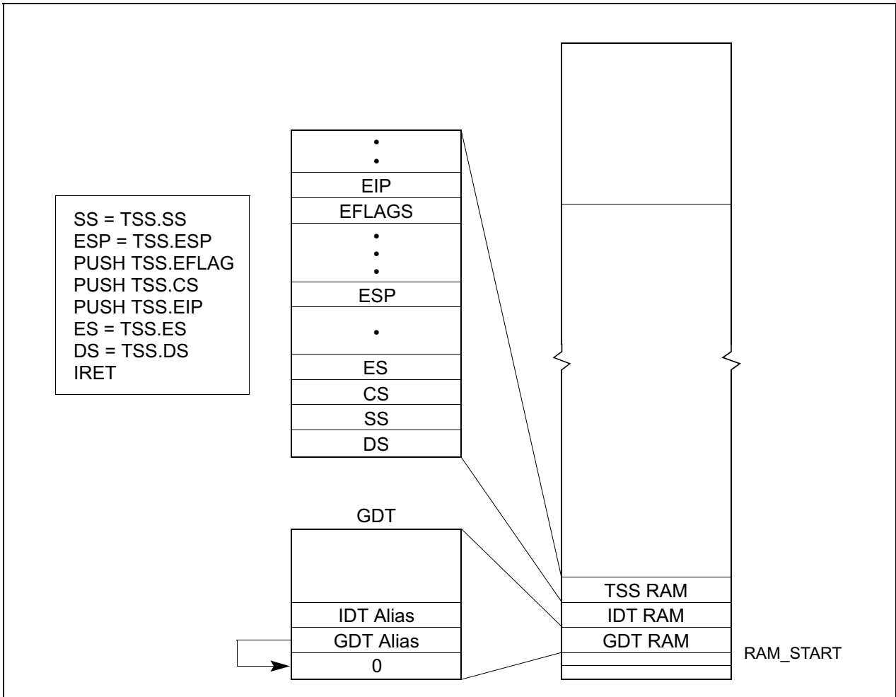
Figure 8-6. Task Switching (Lines 282-296 of List File)
