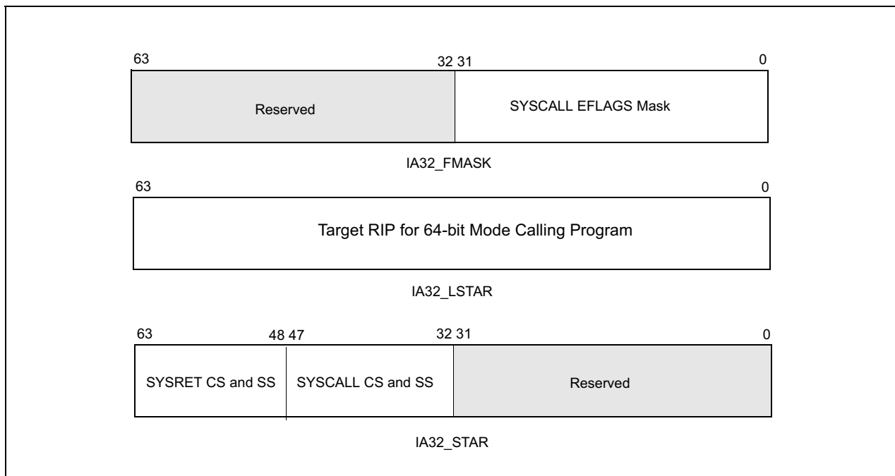
Figure 4-14. MSRs Used by SYSCALL and SYSRET
