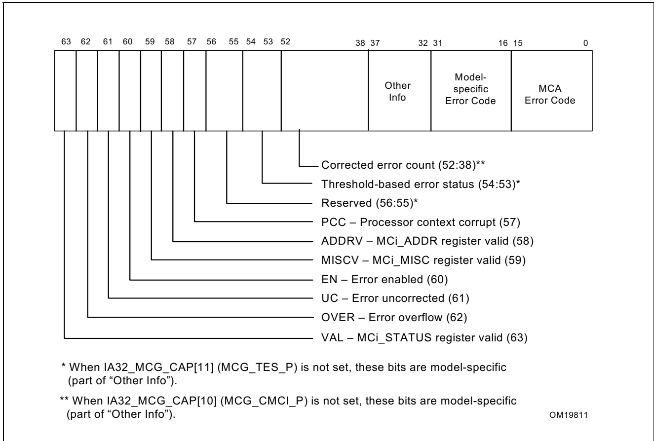
Figure 14-5. IA32_MCi_STATUS Register
