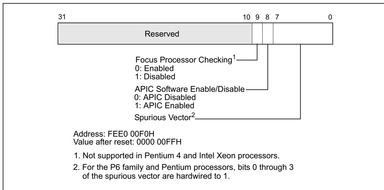
Figure 9-31. Spurious-Interrupt Vector Register (SVR)
