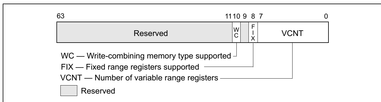
Figure 10-5. IA32_MTRRCAP Register
