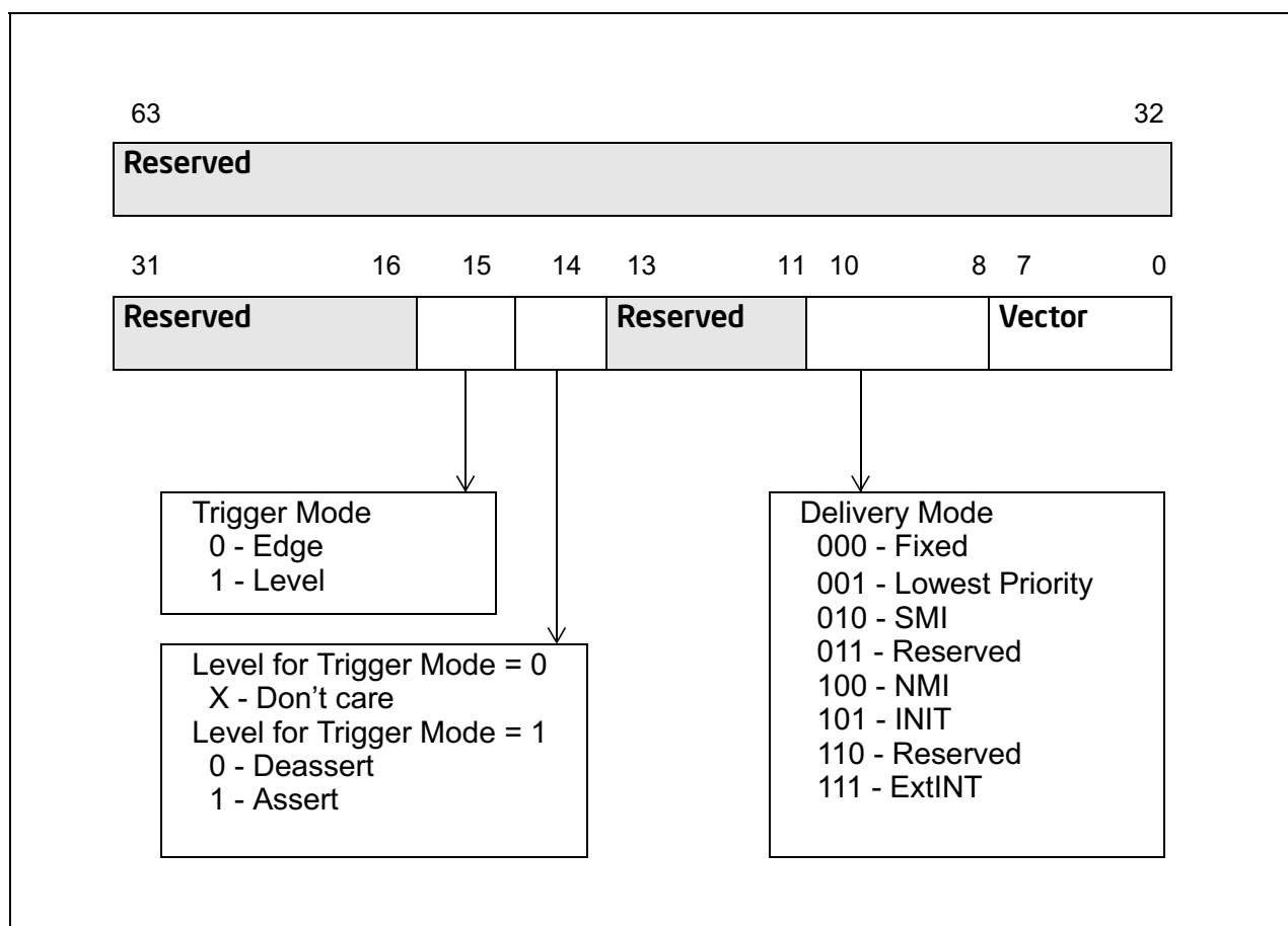
Figure 9-33. Layout of the MSI Message Data Register
