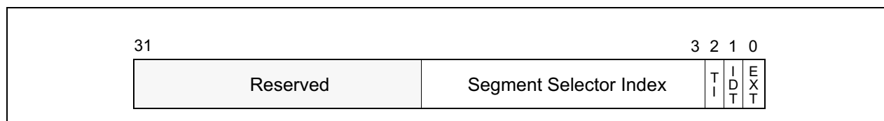
Figure 5-6. Error Code
