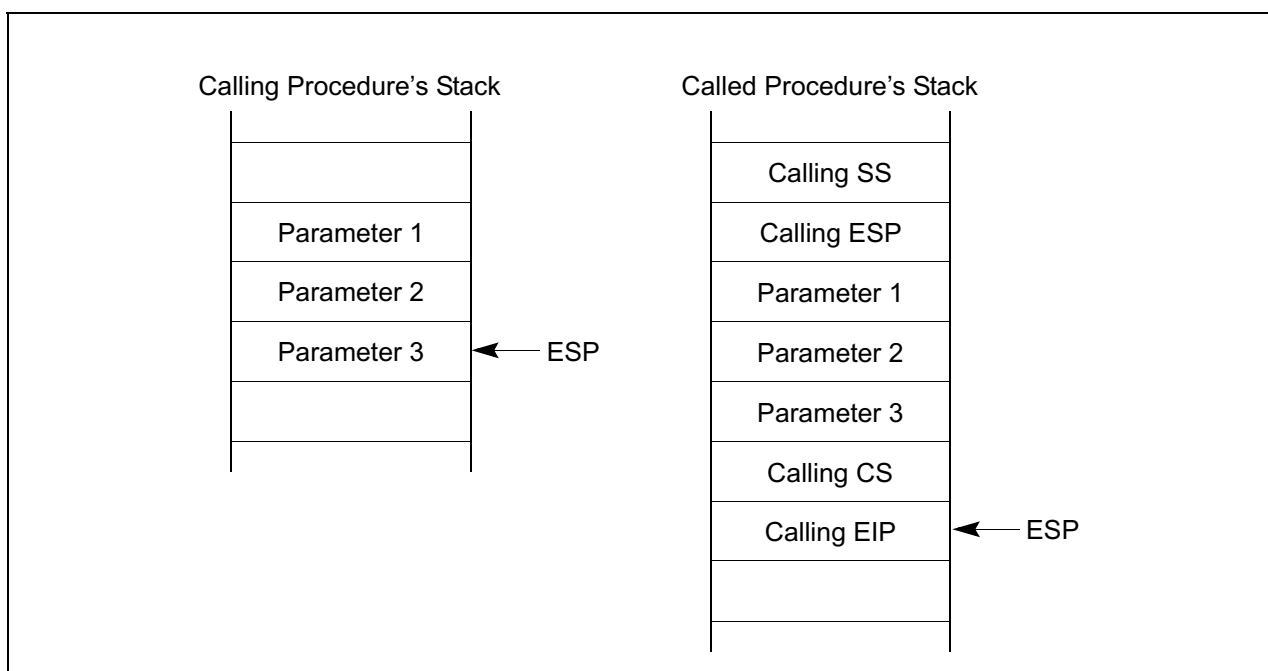
Figure 4-13. Stack Switching During an Interprivilege-Level Call
