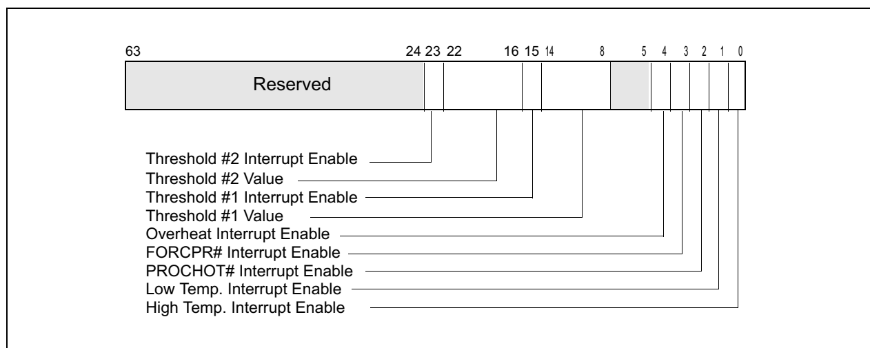
Figure 13-11. IA32_THERM_INTERRUPT Register
