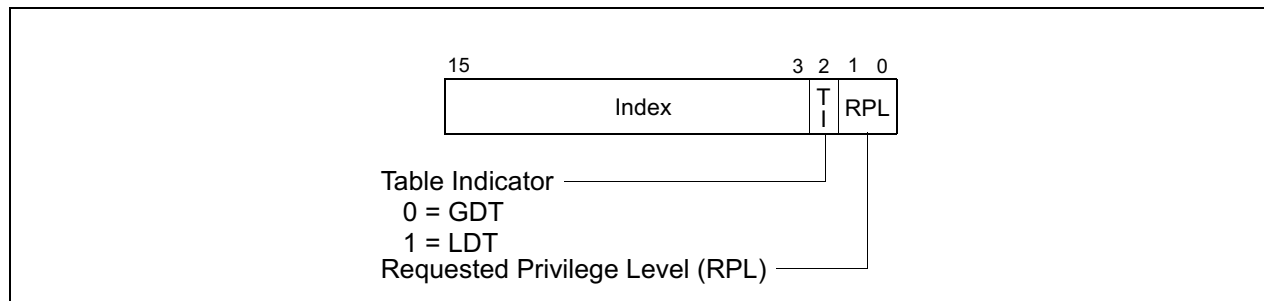
Figure 3-6. Segment Selector
