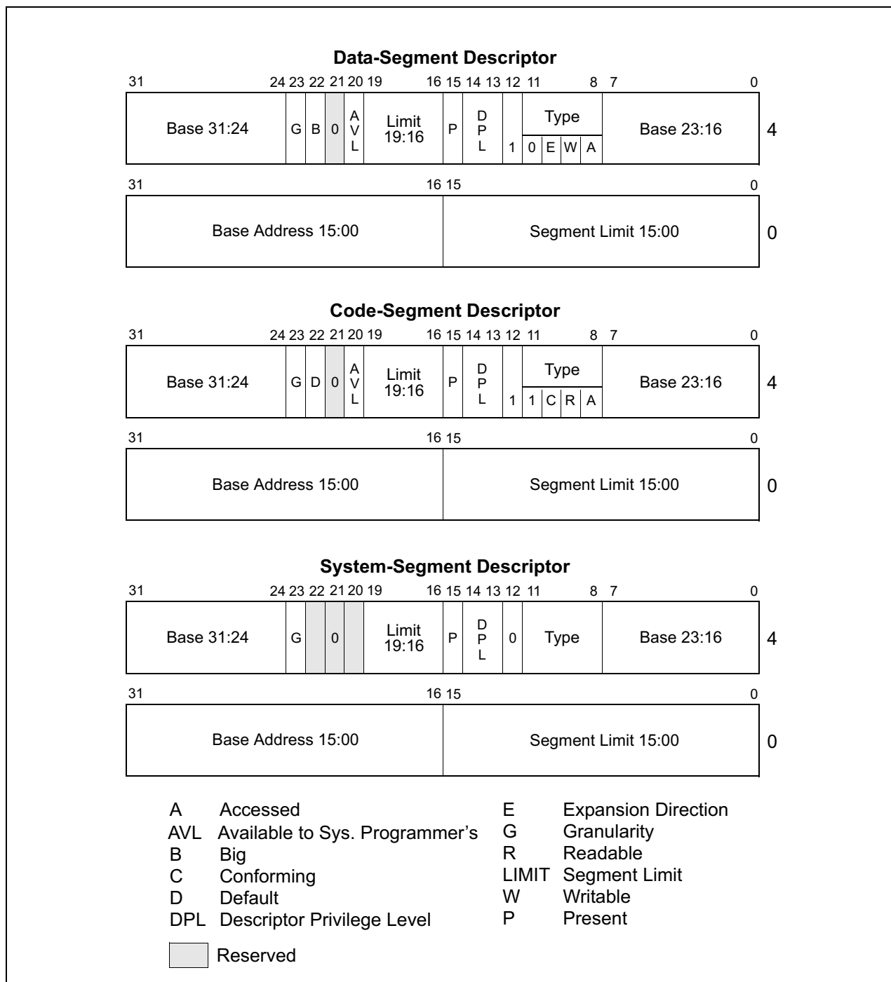
Figure 4-1. Descriptor Fields Used for Protection
