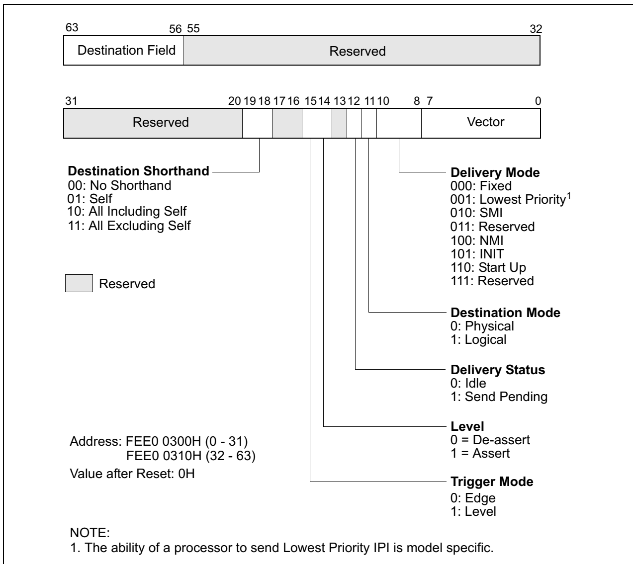
Figure 9-17. Interrupt Command Register (ICR)
