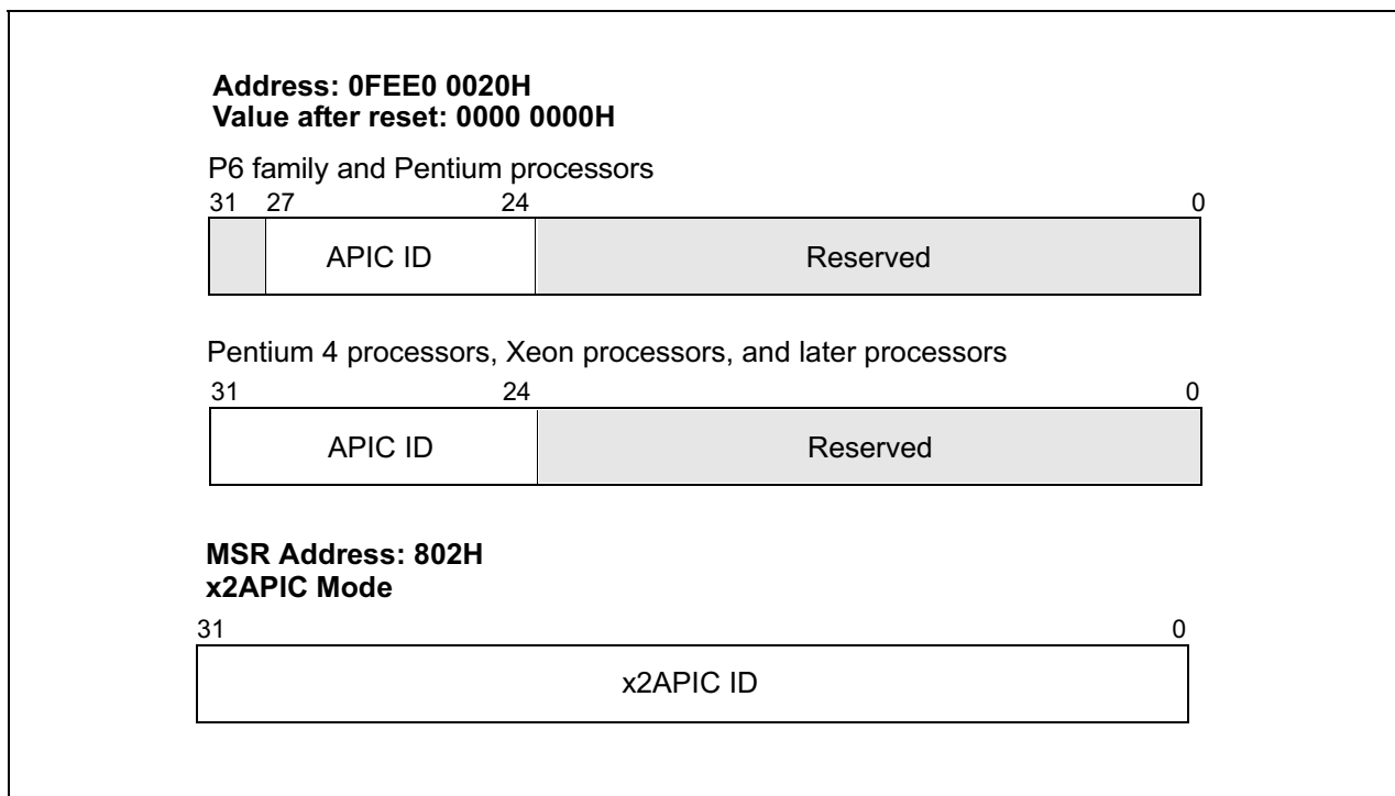
Figure 9-6. Local APIC ID Register
