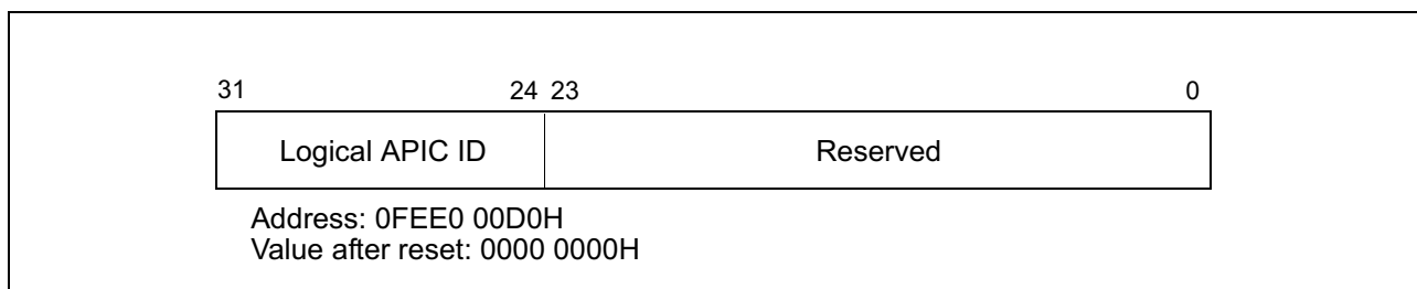
Figure 9-19. Logical Destination Register (LDR)
