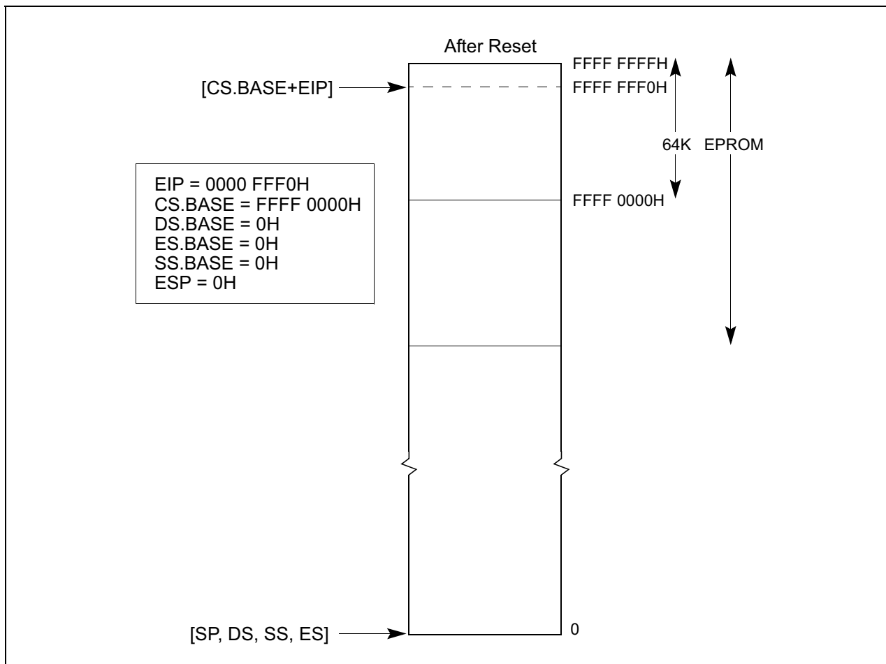
Figure 8-3. Processor State After Reset
