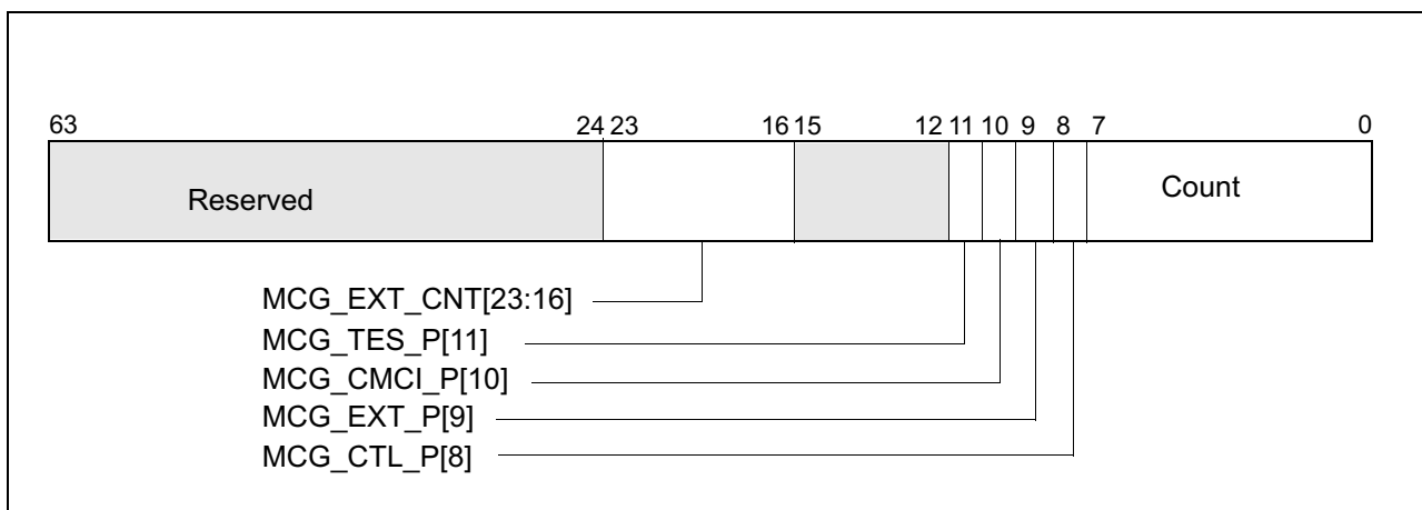
Figure 14-2. IA32_MCG_CAP Register
