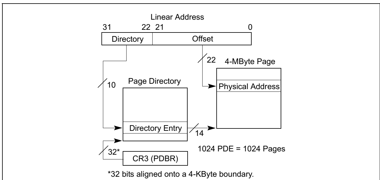
Figure 3-22. Linear Address Translation (4-MByte Pages)
