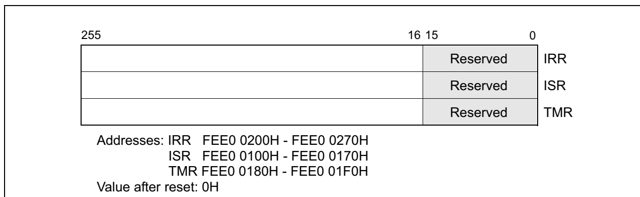
Figure 9-28. IRR, ISR and TMR Registers
