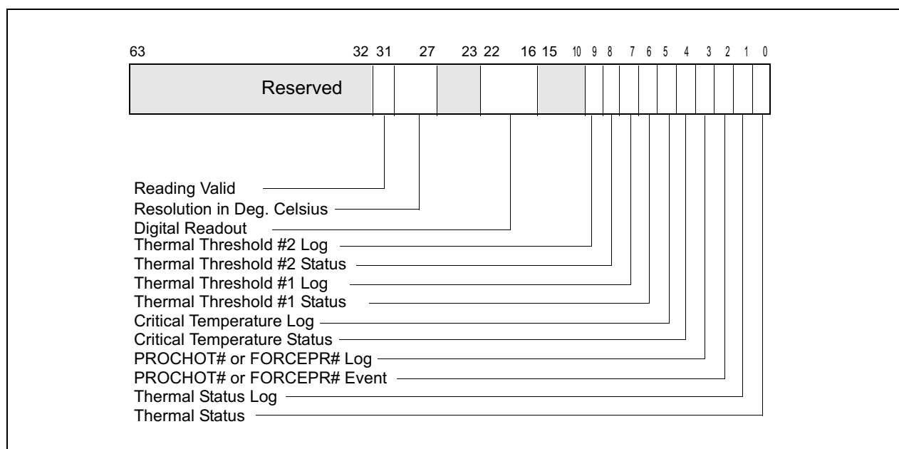
Figure 13-10. IA32_THERM_STATUS Register
