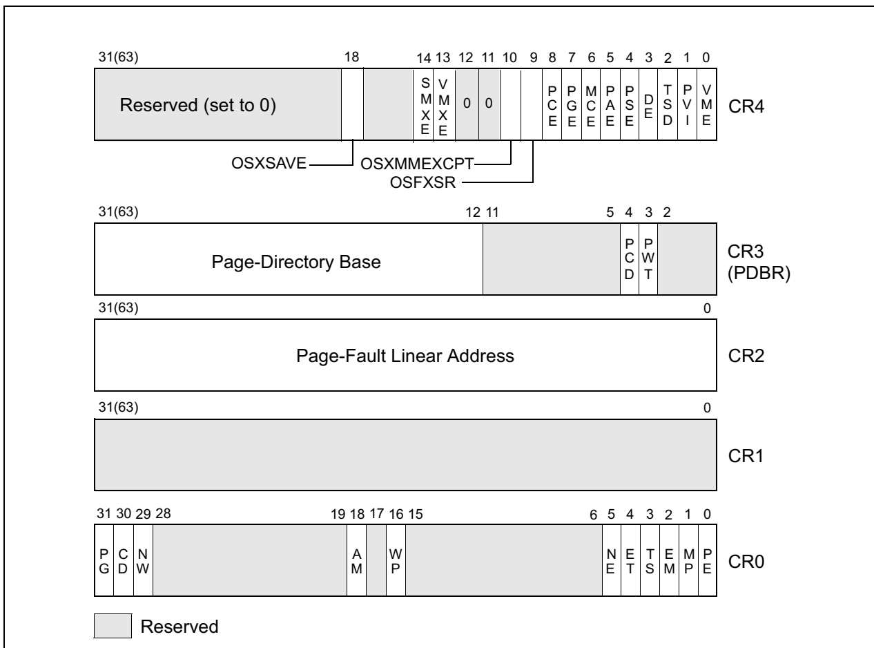
Figure 2-6. Control Registers
