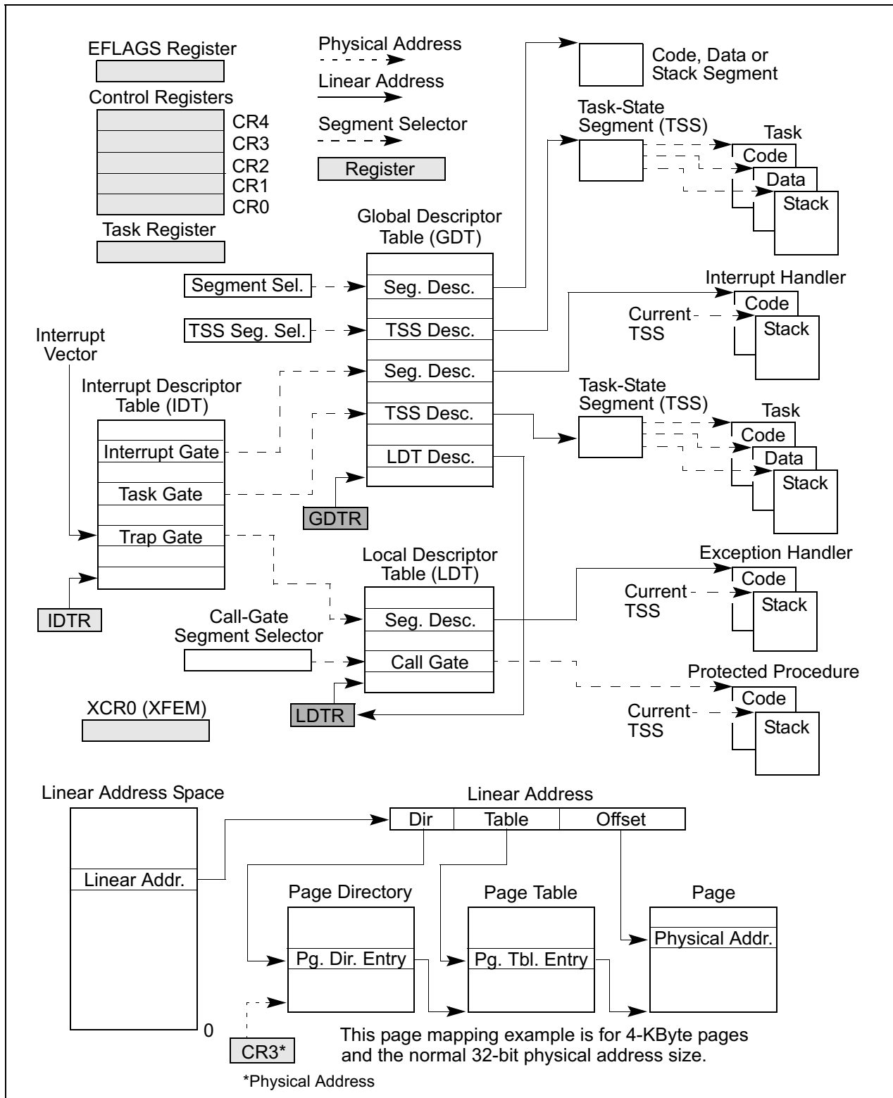
Figure 2-1. IA-32 System-Level Registers and Data Structures
