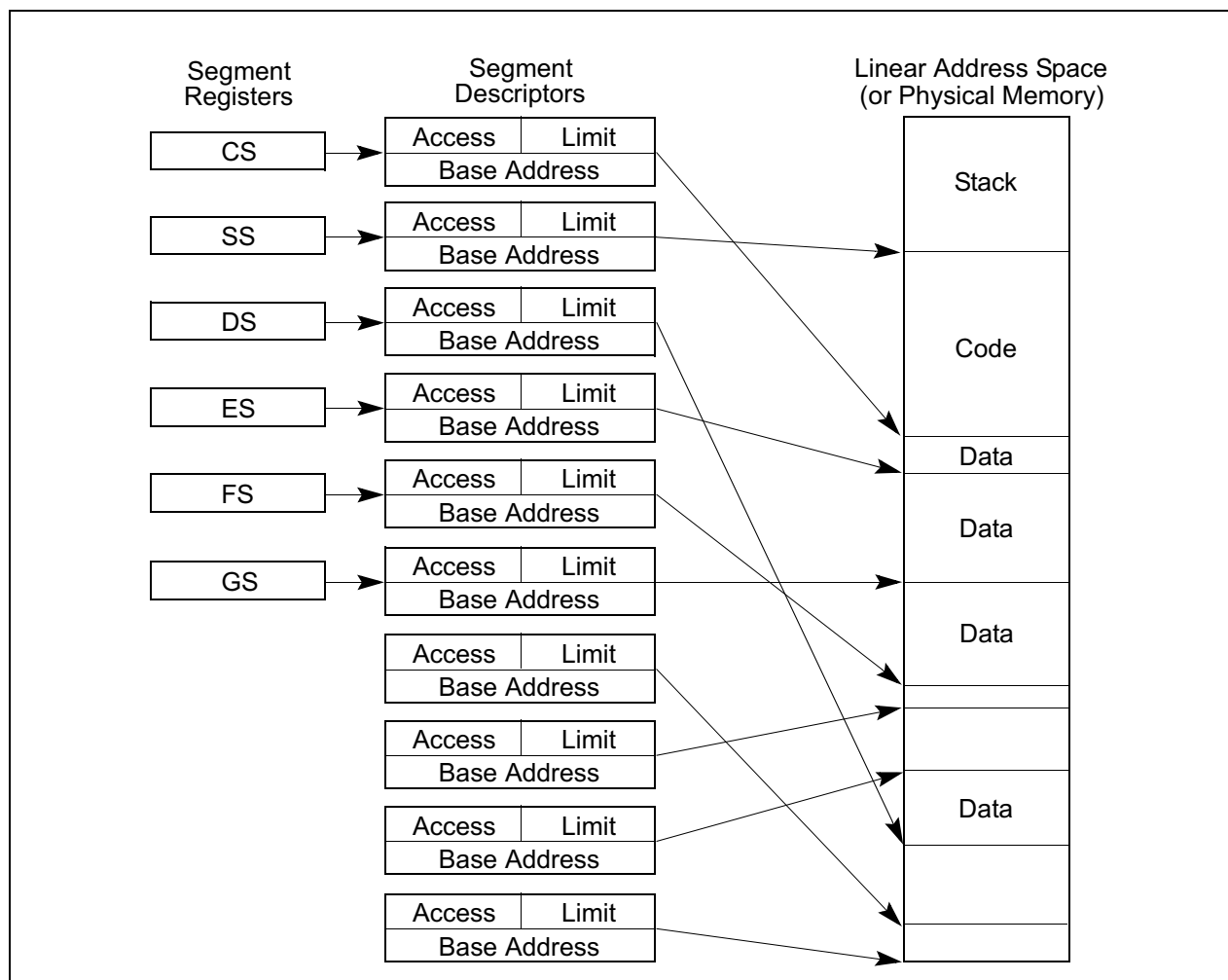
Figure 3-4. Multi-Segment Model
